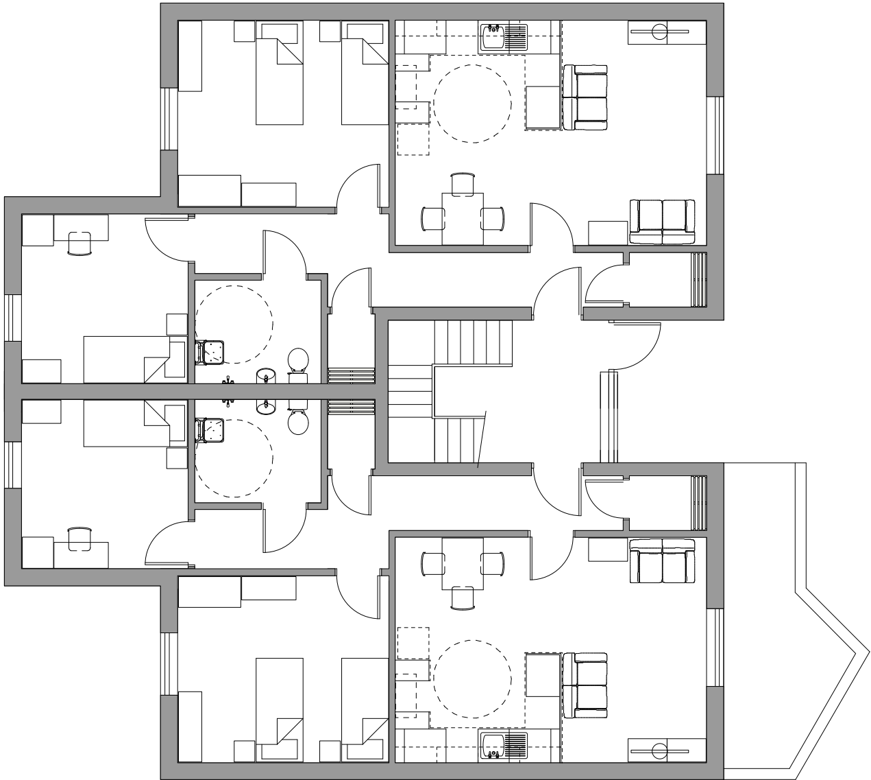
Apartment Type C
