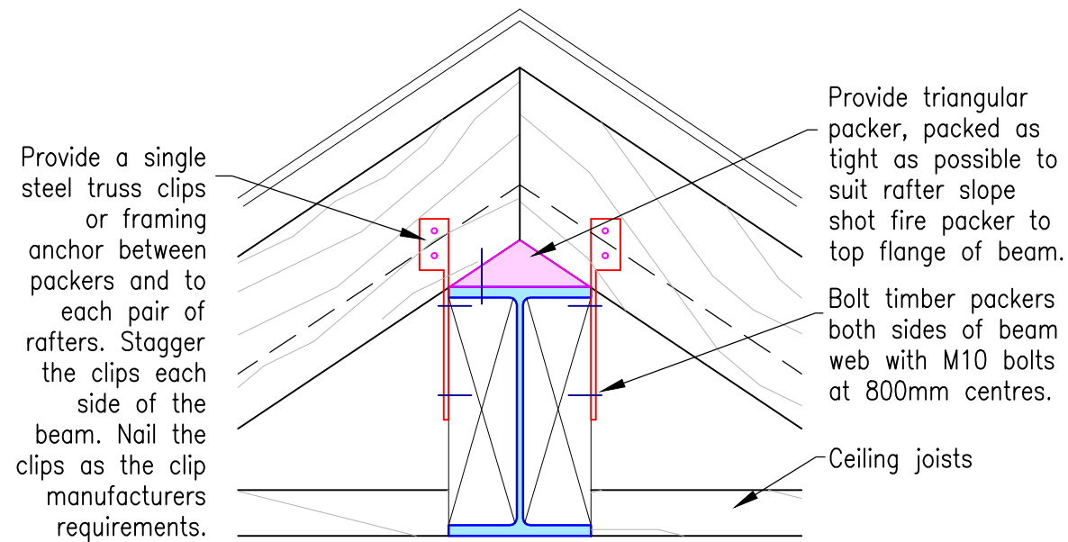
Ridge Beam Detail
