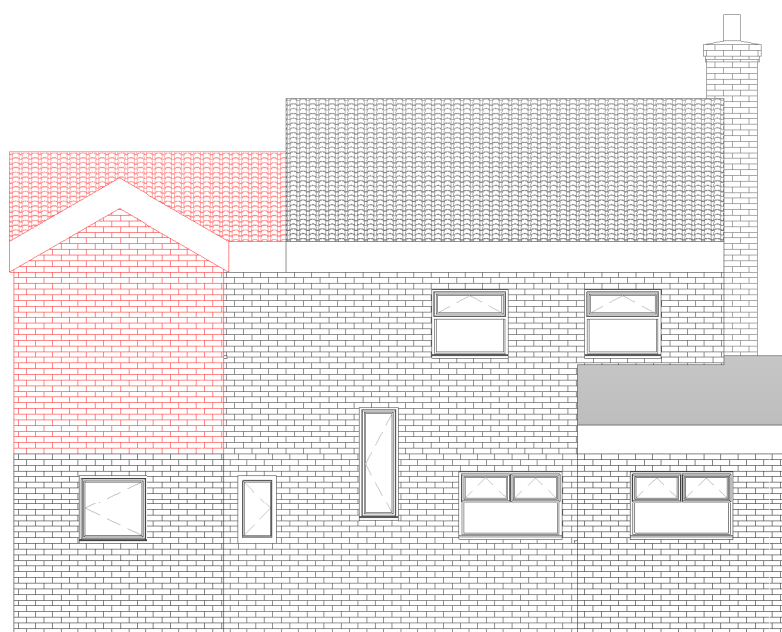
2 Proposed South Elevation 1 : 100
