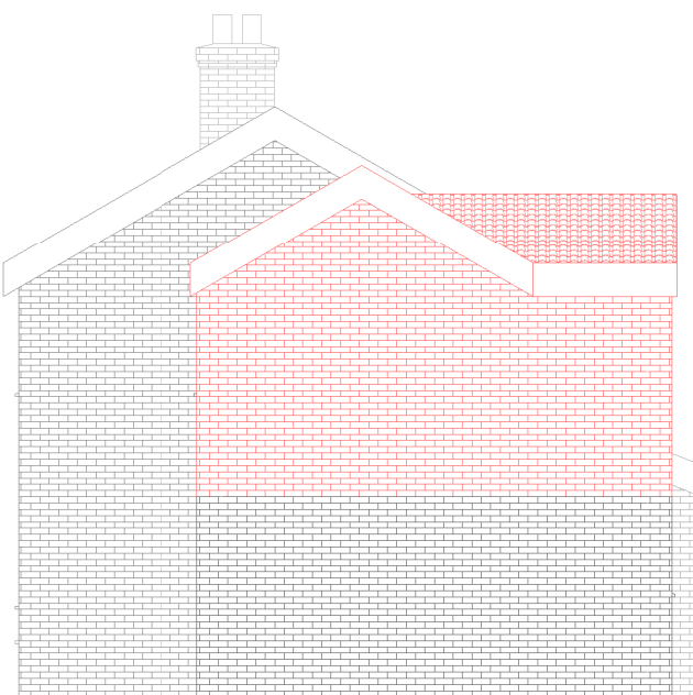
4 Proposed West Elevation 1 : 100
