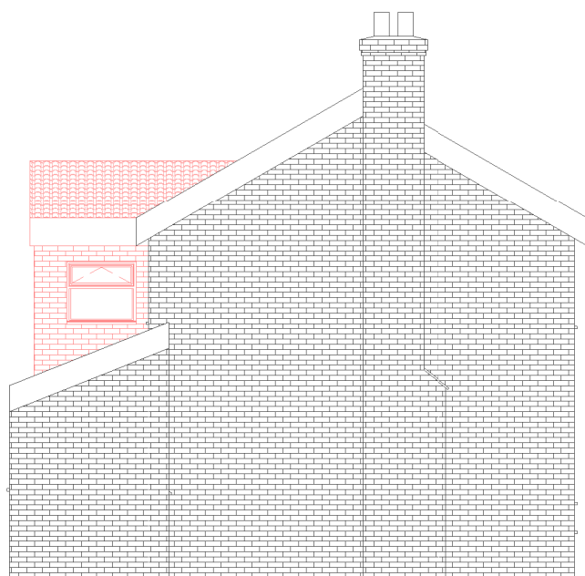
3 Proposed East Elevation 1 : 100
