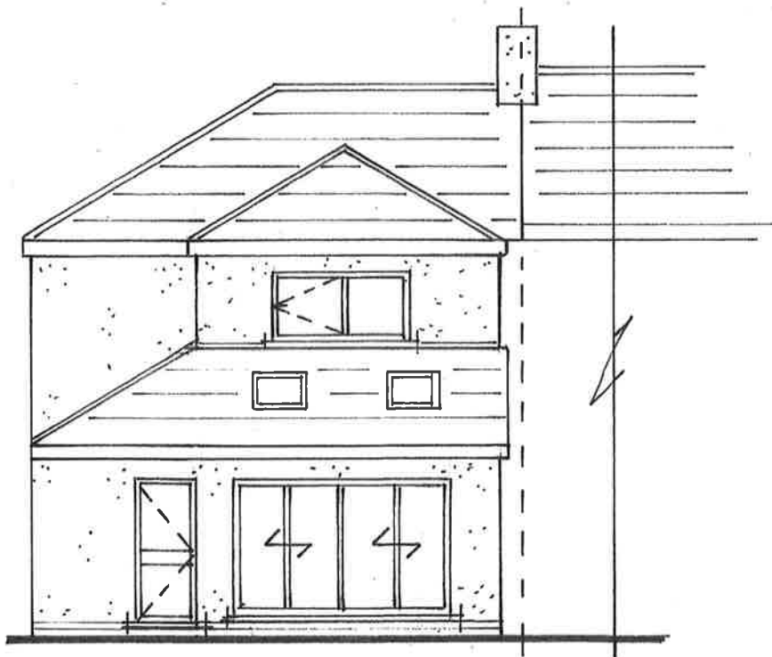
PROPOSED REAR
