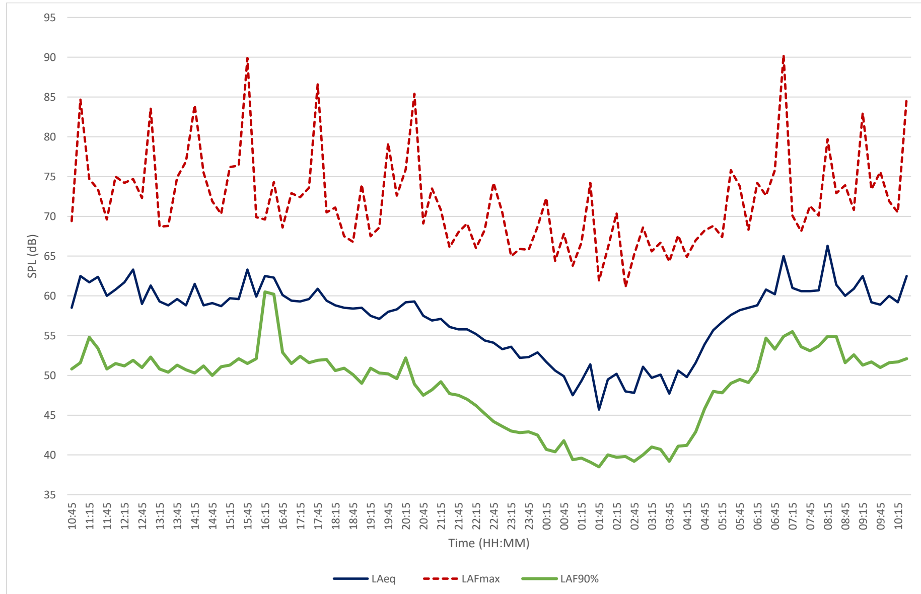
Figure B.3 – Time History at Position A (Thursday 1 st August 2019 to Friday 2 nd August 2019)
