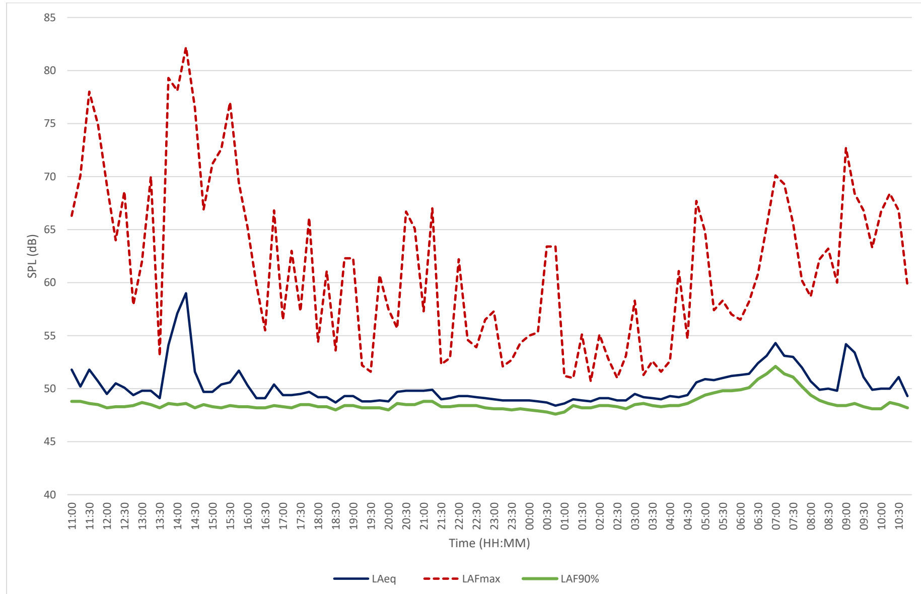
Figure B.5 - Time History at Position C (Thursday 1 st August 2019 to Friday 2 nd August 2019)
