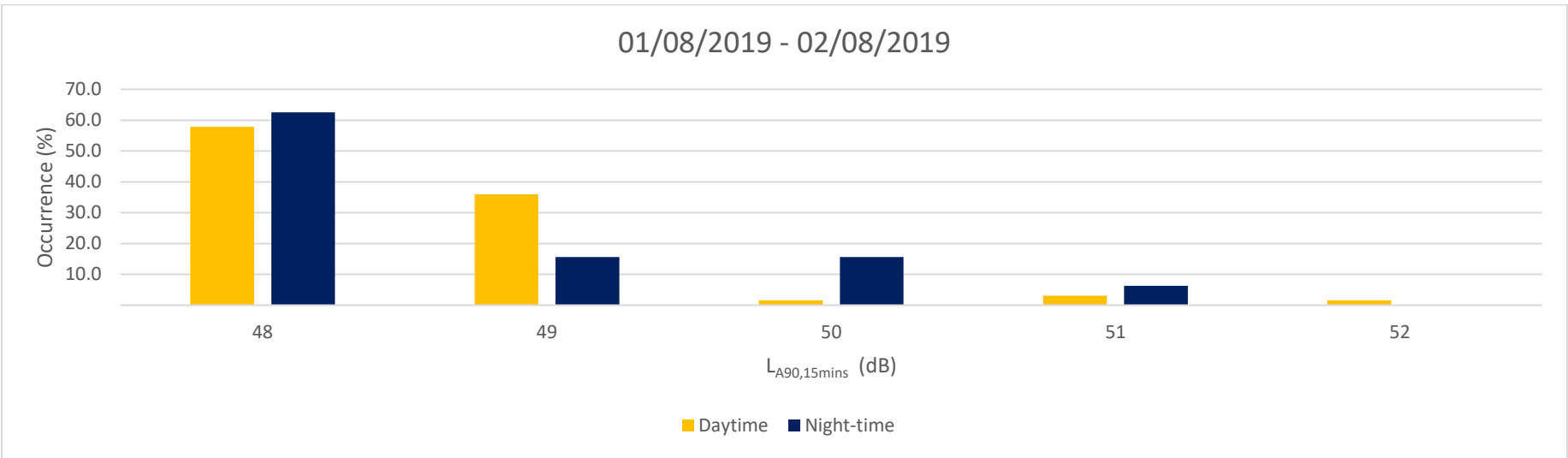
Figure B.8 – Most Commonly Occurring Background Noise Level At Position C
