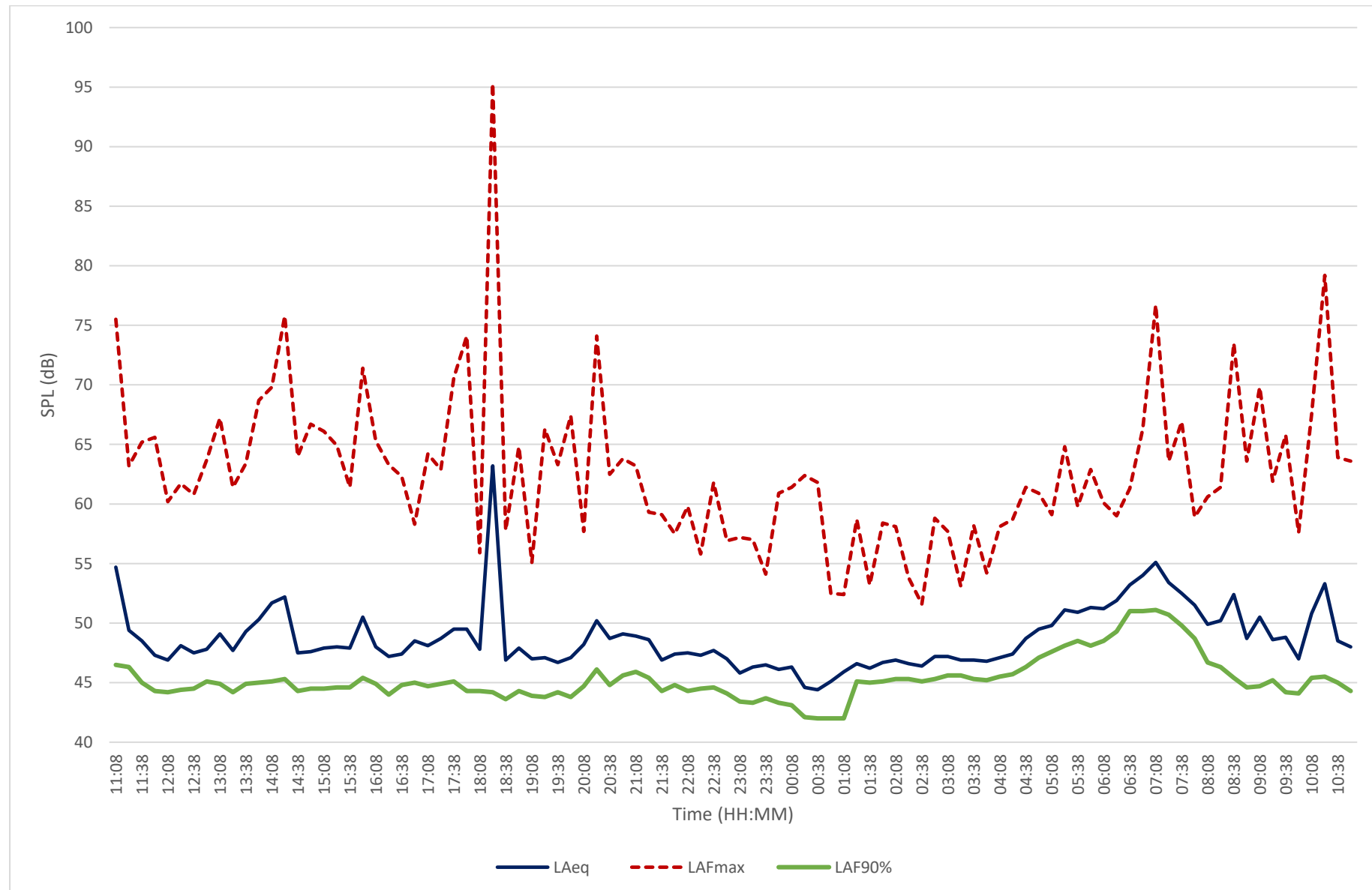
Figure B.4 - Time History at Position B (Thursday 1 st August 2019 to Friday 2 nd August 2019)
