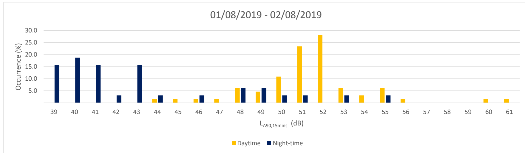
Figure B.6 – Most Commonly Occurring Background Noise Level at Position A
