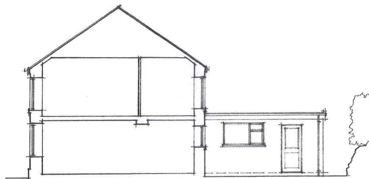
SECTIONAL SIDE ELEVATION
