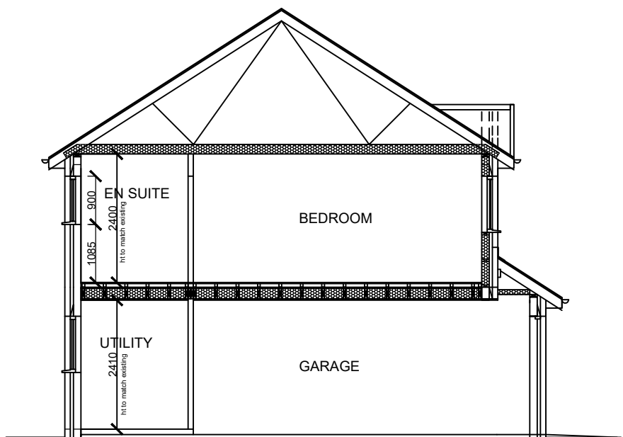
Existing Foundations to be exposed & checked for suitability via trial holes excavated as required by LA Building Control PROPOSED SECTION A-A
