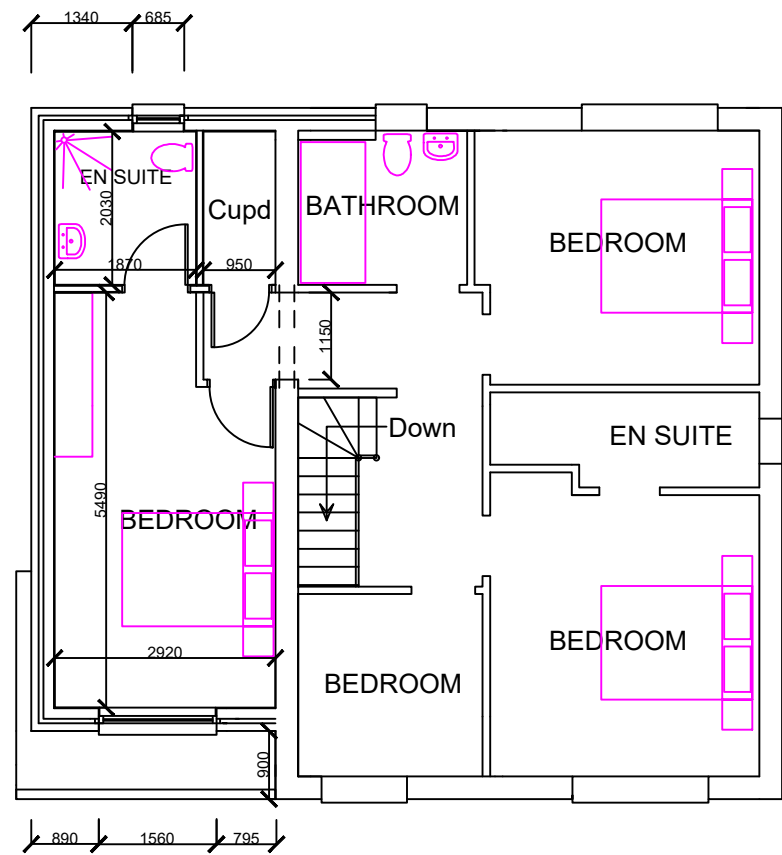
PROPOSED F.F. PLAN
