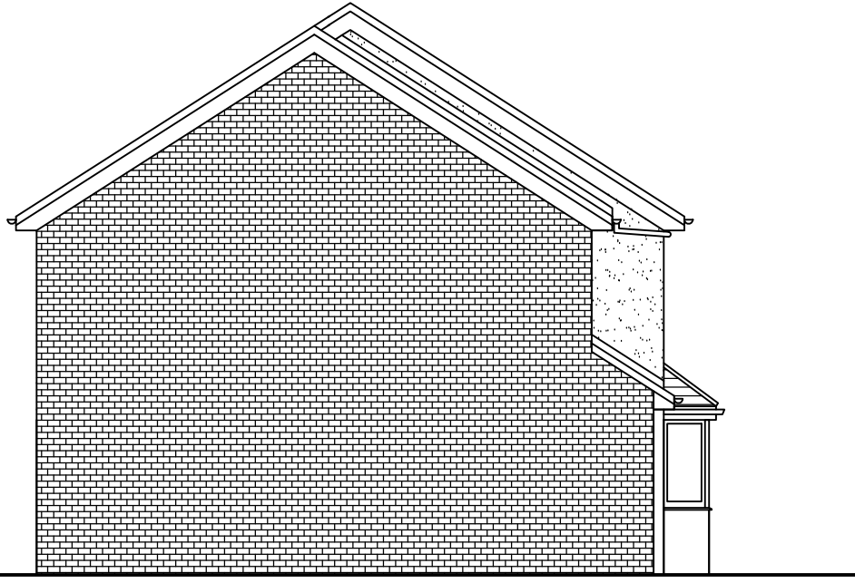
PROPOSED END ELEVATION
