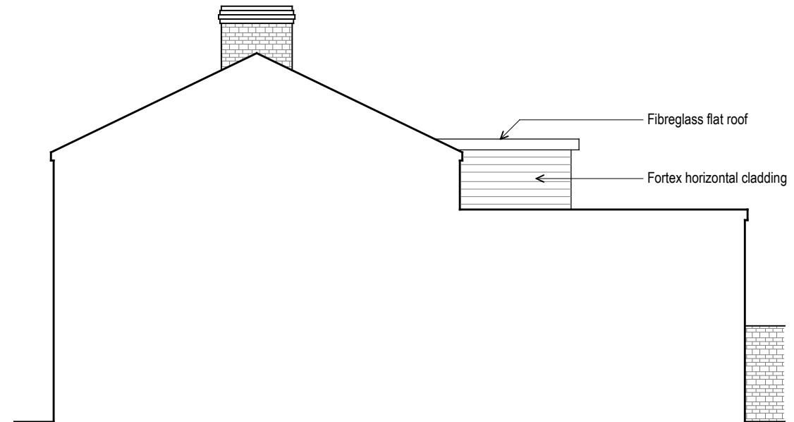
South-East Sectional Elevation
