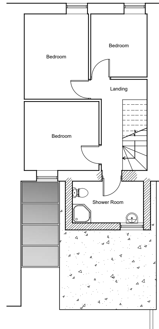
First Floor Plan Scale: 1:100 @ A3
