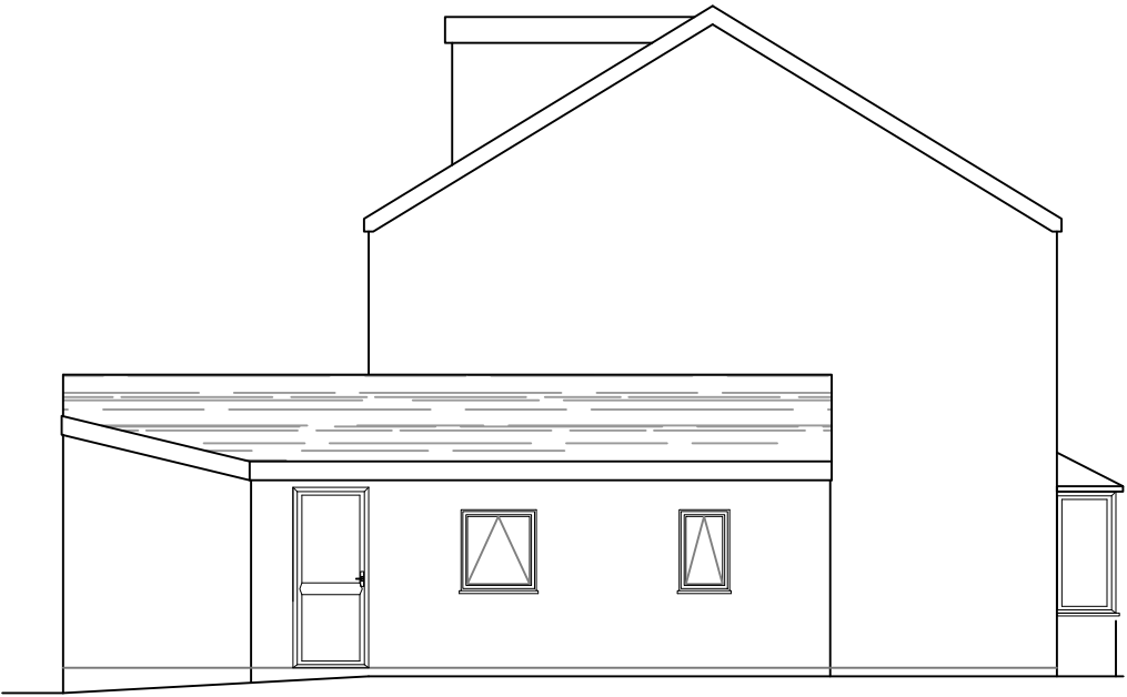
Proposed elevation on 'B' Scale - 1:100
