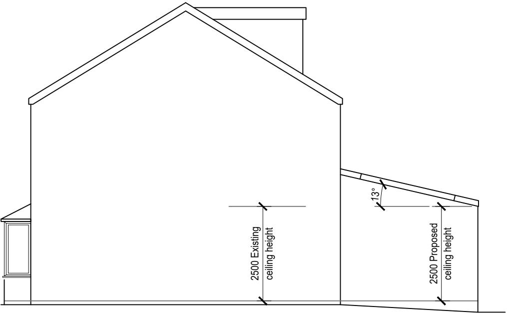
Proposed elevation on 'A' Scale - 1:100
