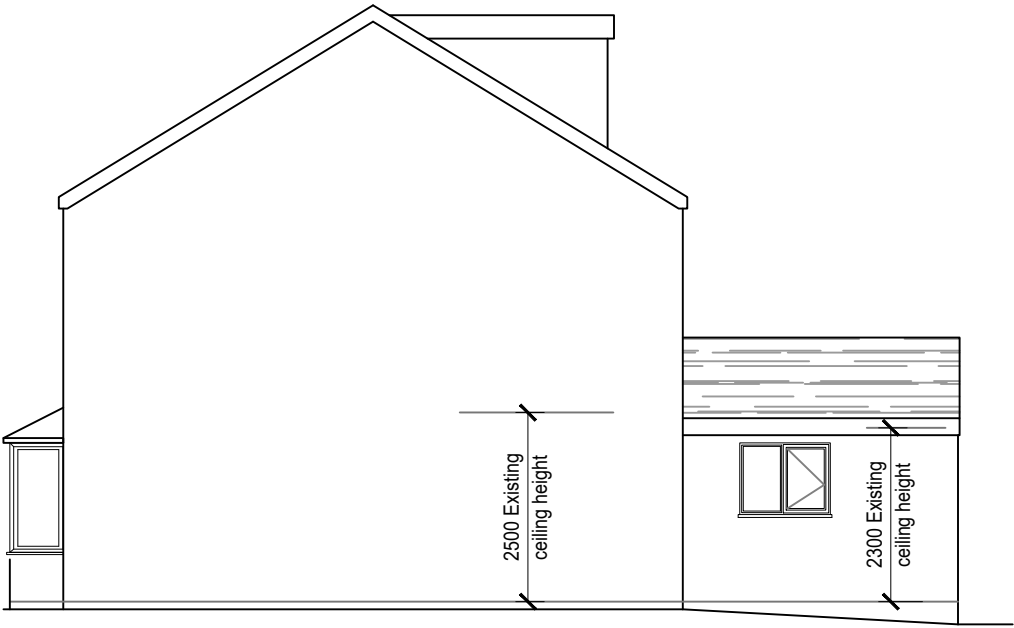
Existing elevation on 'A' Scale - 1:100
