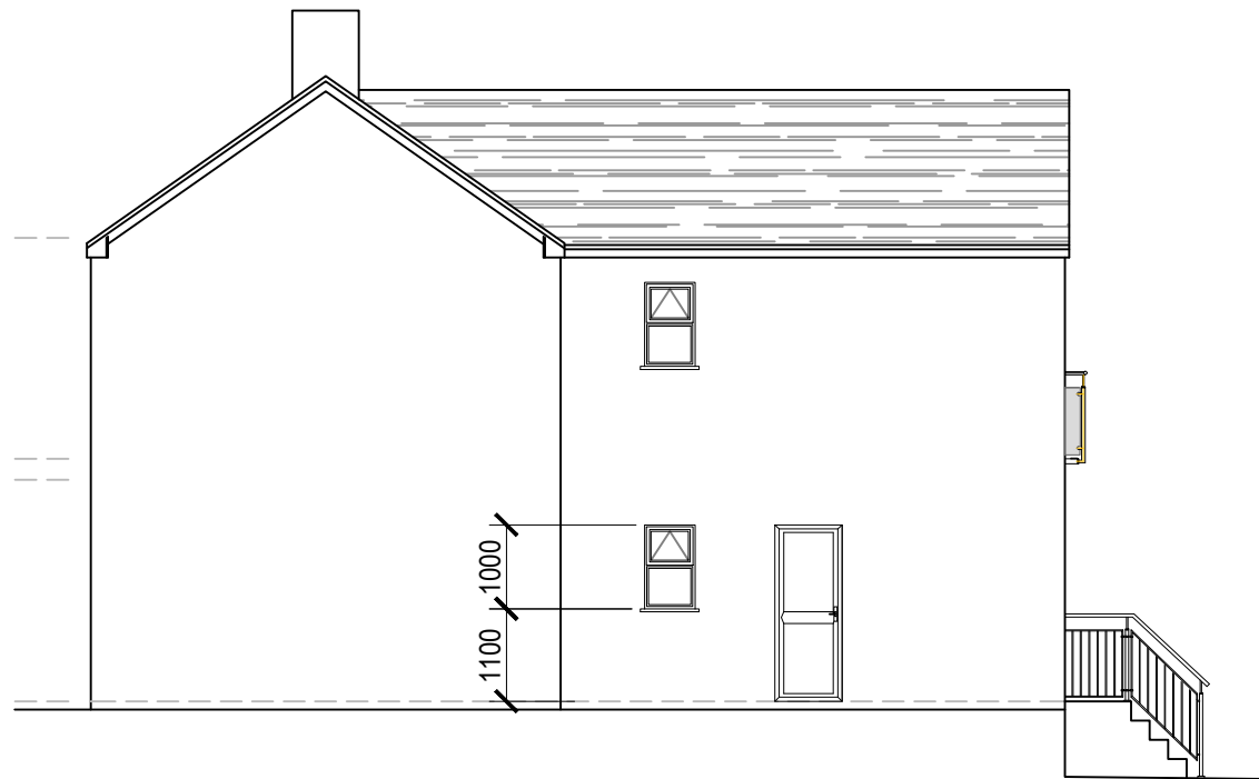
Proposed elevation on 'B' Scale - 1:100
