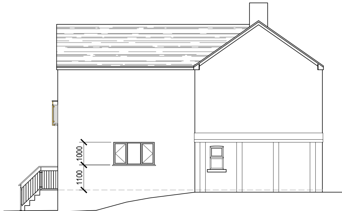
Proposed elevation on 'A' Scale - 1:100
