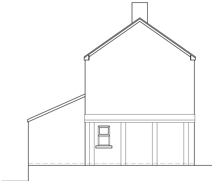
Existing elevation on 'A' Scale - 1:100
