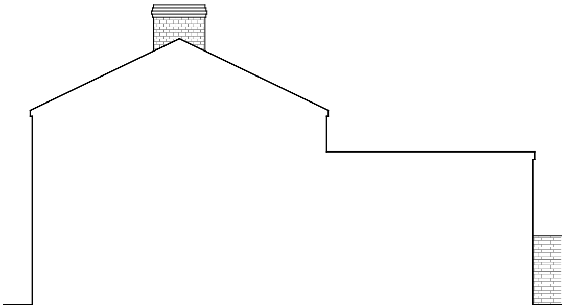
South-East Sectional Elevation Scale: 1:100 @ A3
