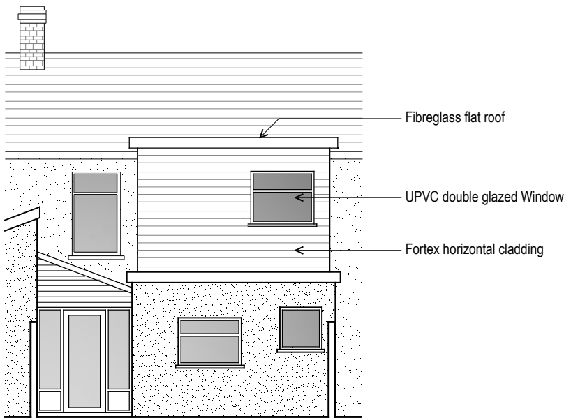
North-East Elevation
