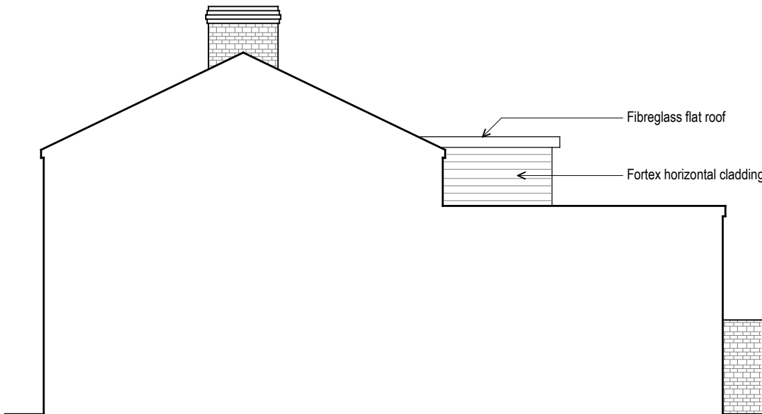
South-East Sectional Elevation
