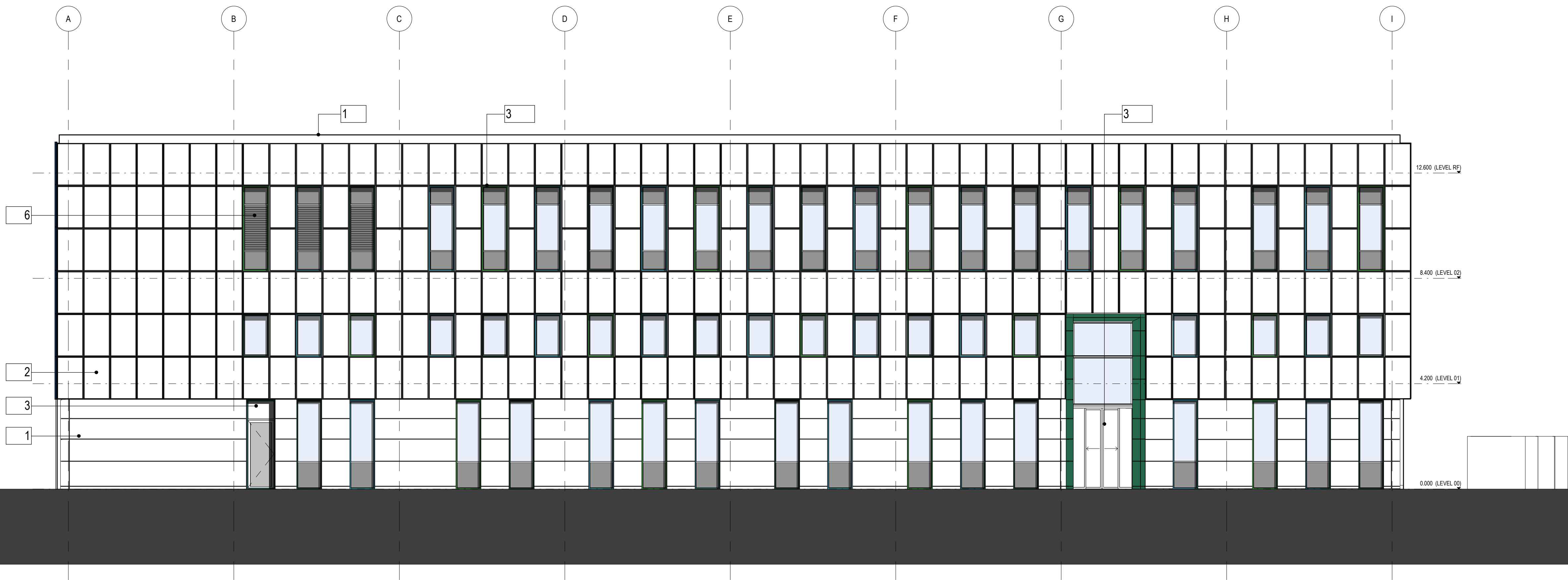
Elevation 1 Planning 1 : 100
