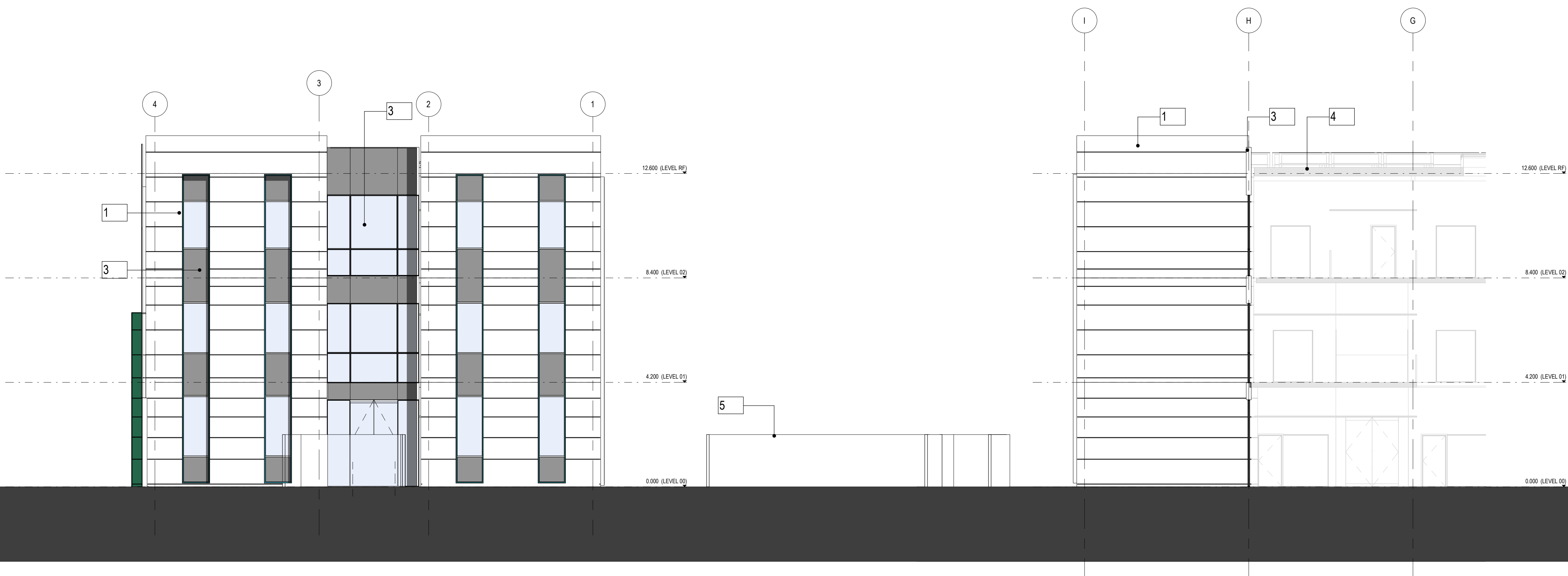
Elevation 2 Planning 1 : 100
