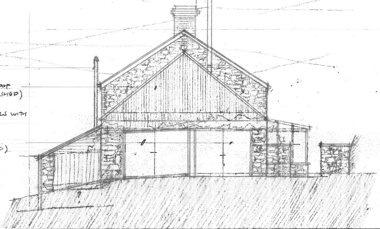
NORTH WEST ELEVATION ~ SCALE 1:100 @ A3
