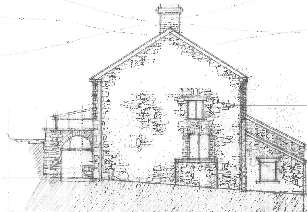
SOUTH EAST ELEVATION ~ SCALE 1:100 @ A3
