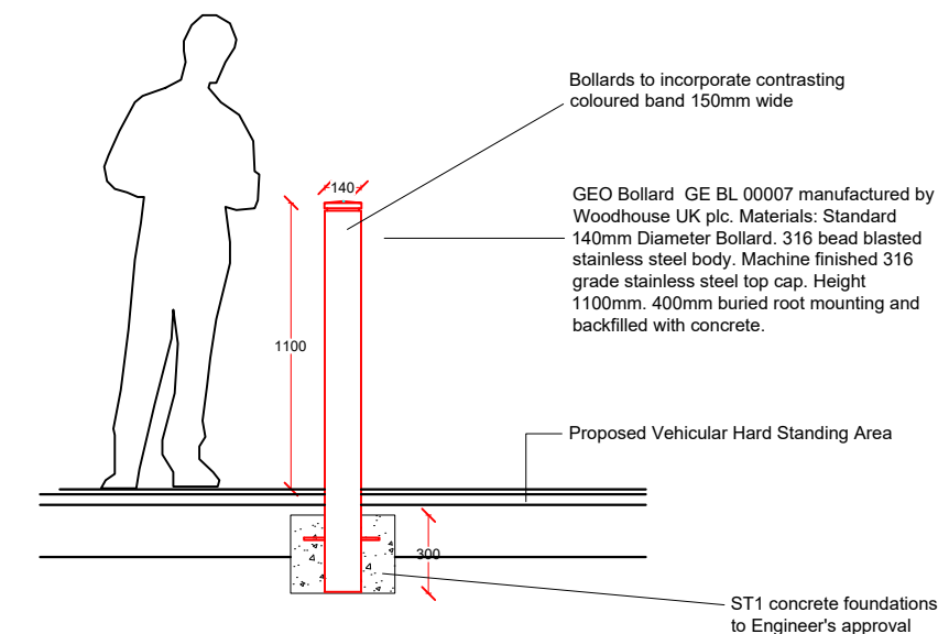
Brushed Stainless Steel Bollard Details
