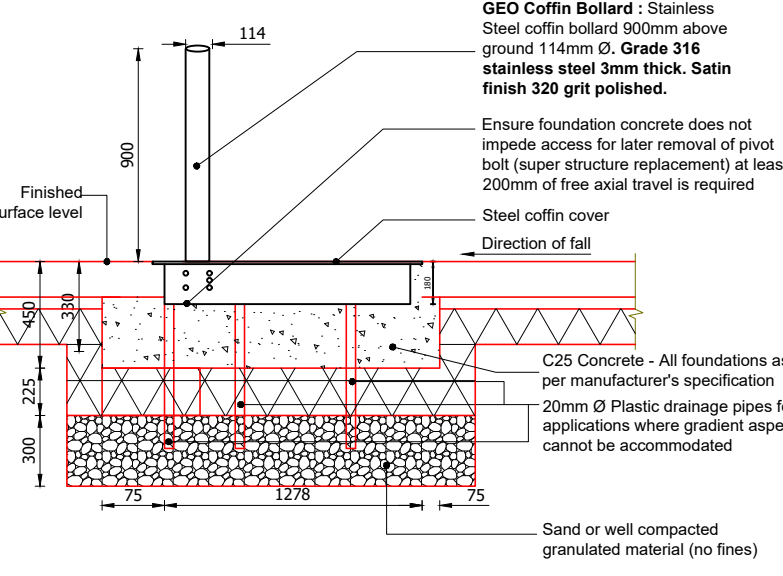
Drop Down 'Coffin' Bollard Details
