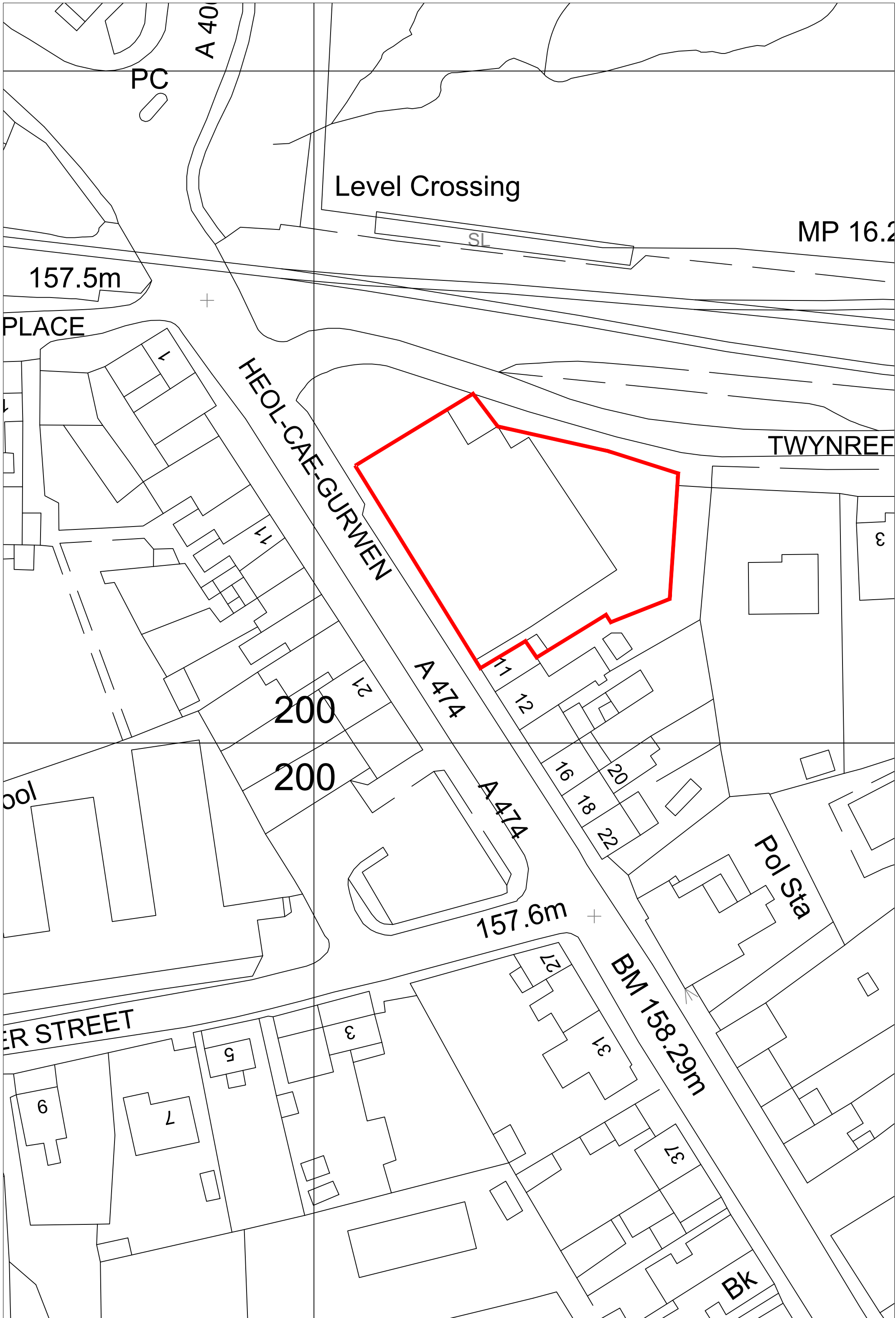
SITE LOCATION PLAN Scale 1:1250
