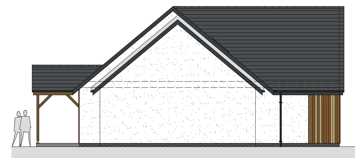
east elevation
