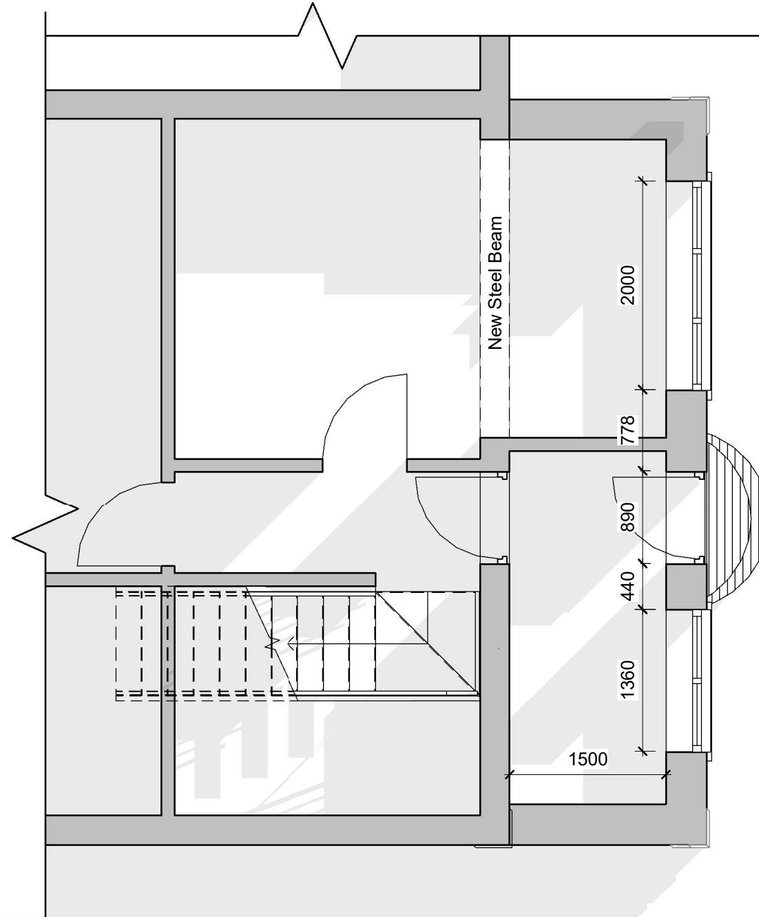
2 Proposed Ground Floor 1 : 50
