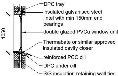
Window Detail
