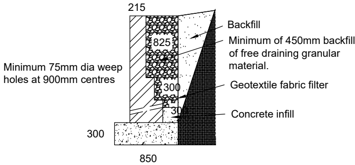
Typical Retaining Wall (Brick)
