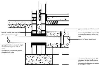
Welsh Water BOS Detail
