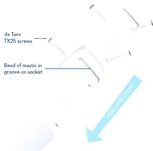
Continuously ventilated/Universal/plain angle ridge
