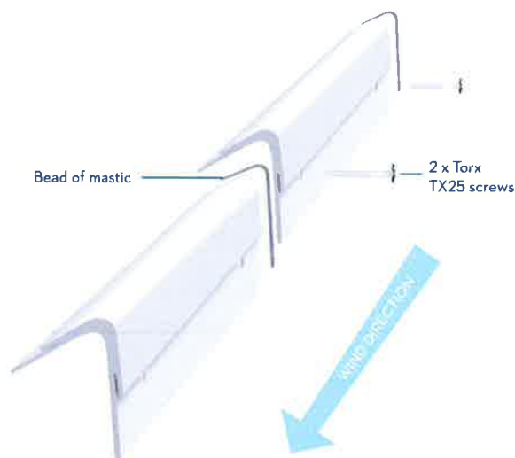
Continuously ventilated monopitch ridge
