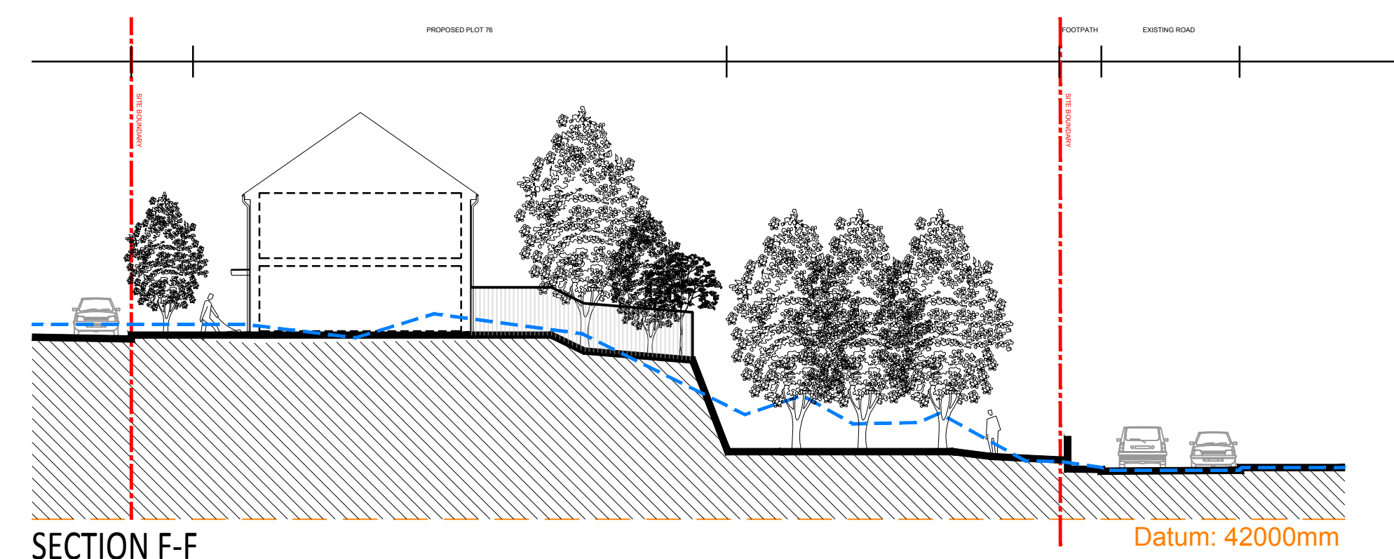
SECTION F-F
