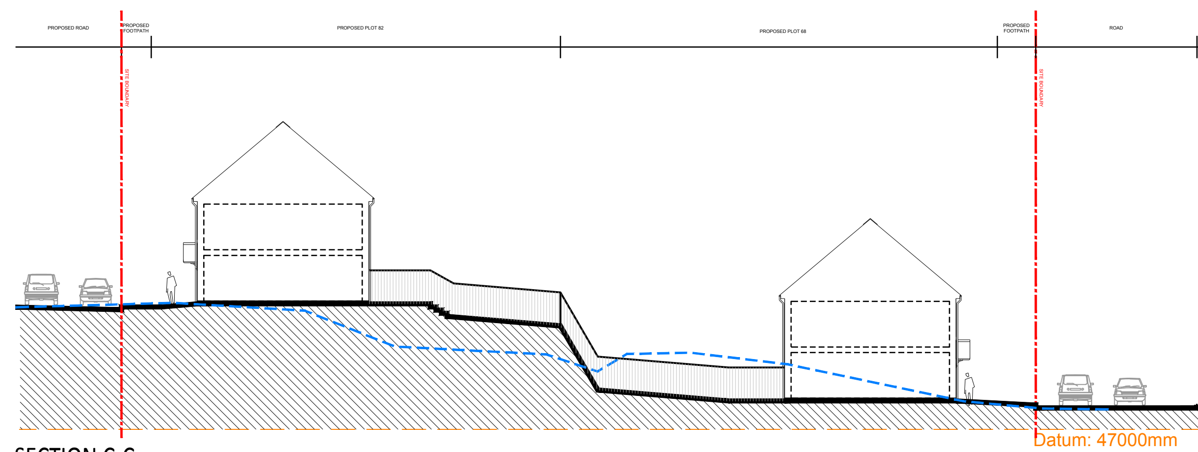
SECTION C-C
