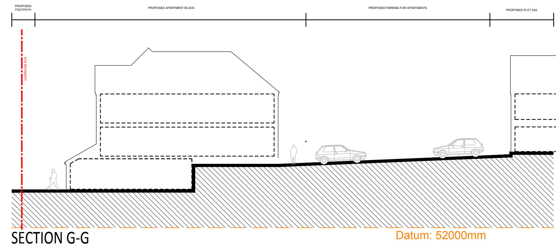
SECTION G-G
