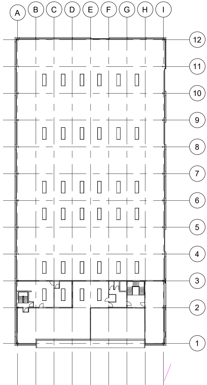
2 Revised Roof Plan 1 : 500
