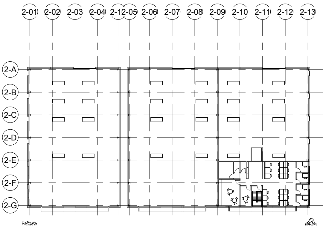
1 Revised First Floor 1 : 500
