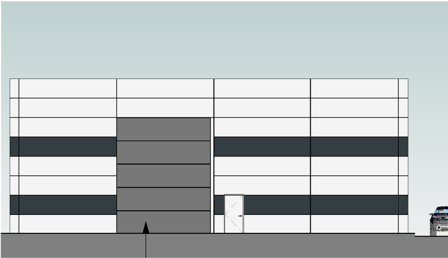
Block 1 West 1 : 200
