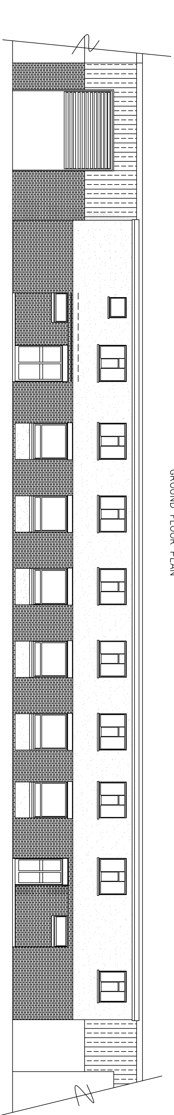
SOUTH ELEVATION
