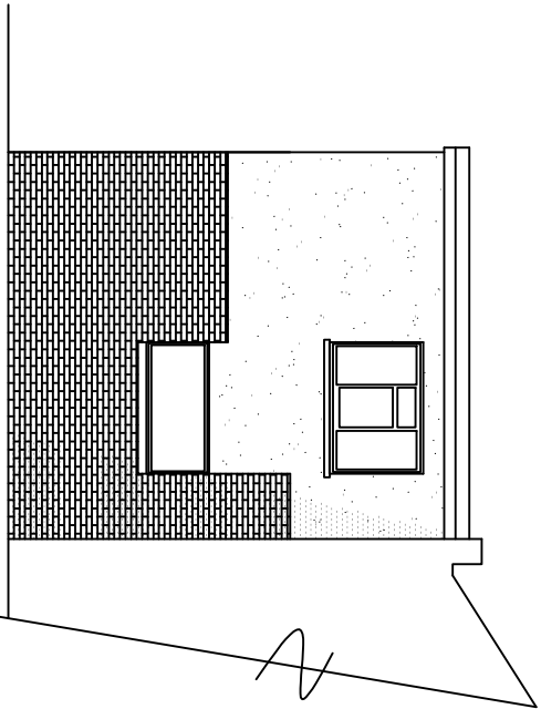
EAST ELEVATION
