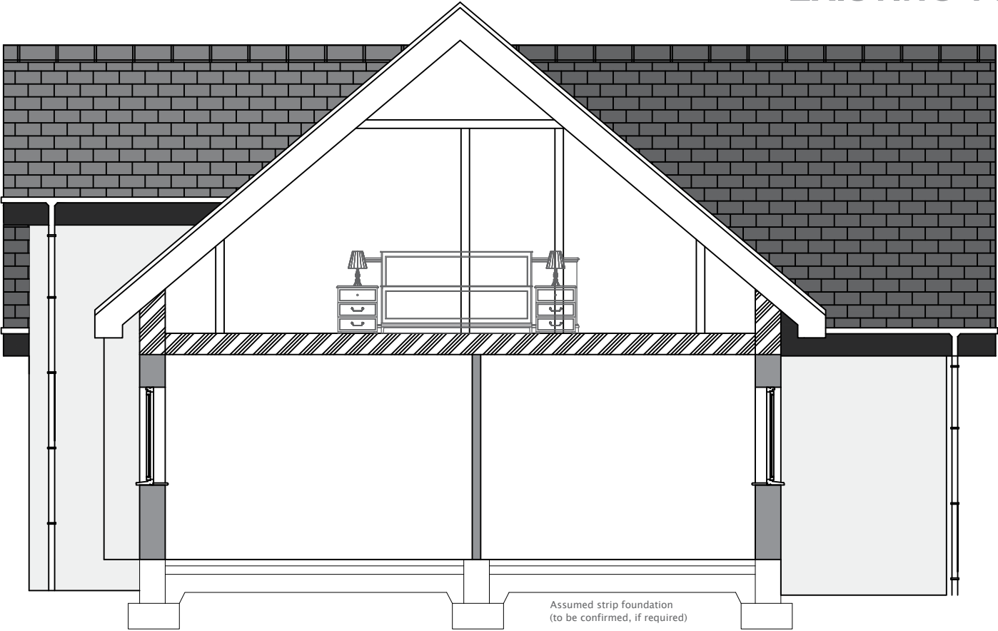
PROPOSED TYPICAL SECTION
