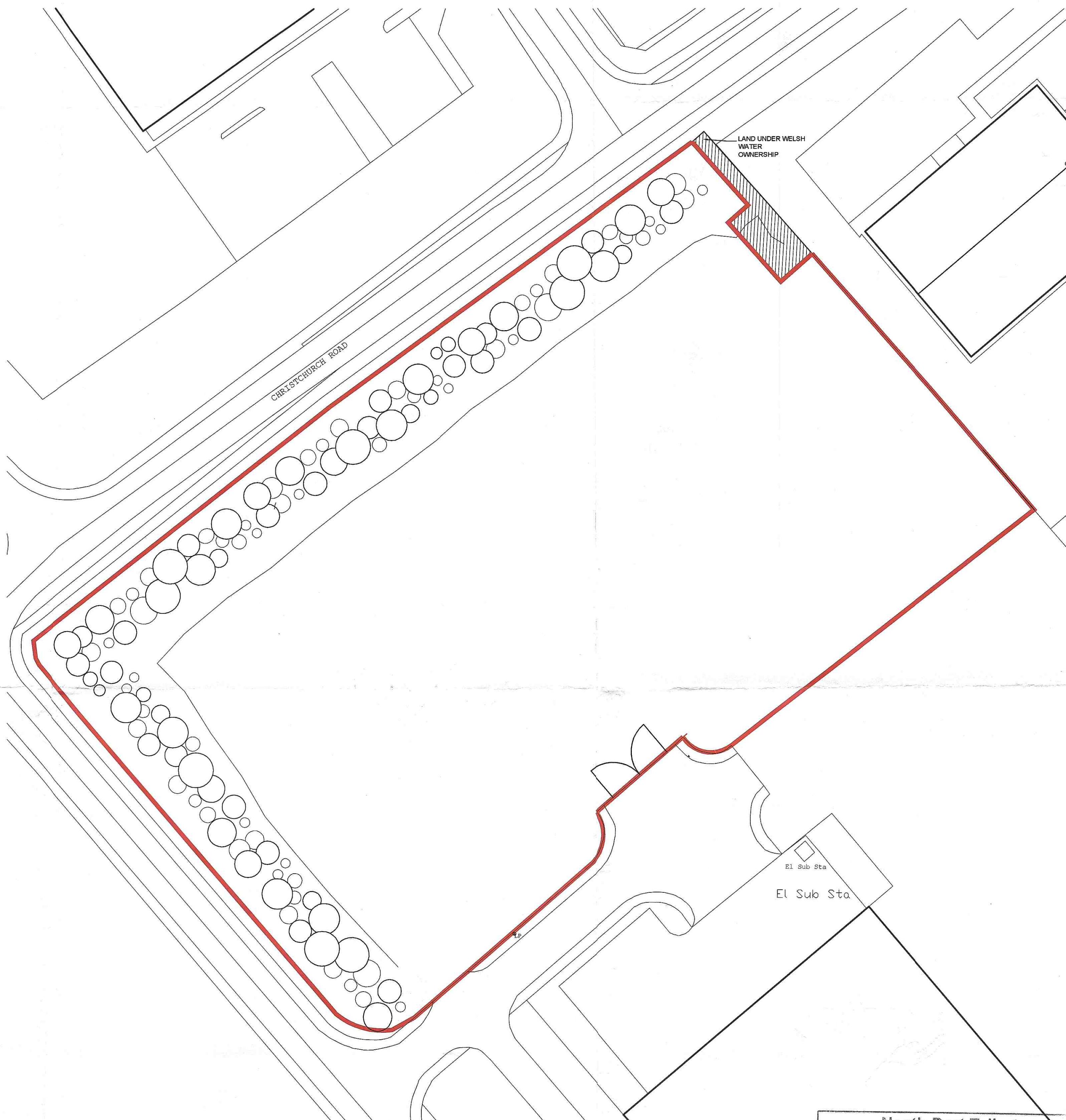
BLOCK PLAN SCALE 1:500 @ A1
