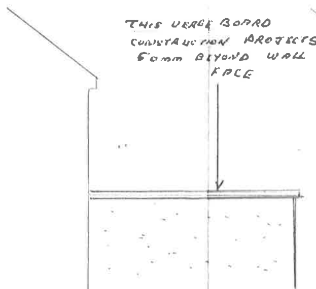
ELEVATION TO NEIGHBOUR EXISTING
