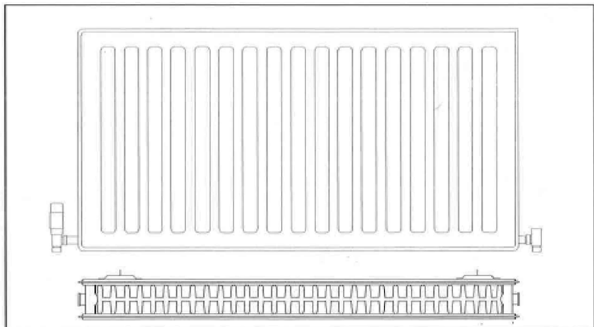
Plan & Elevation of Radiators
