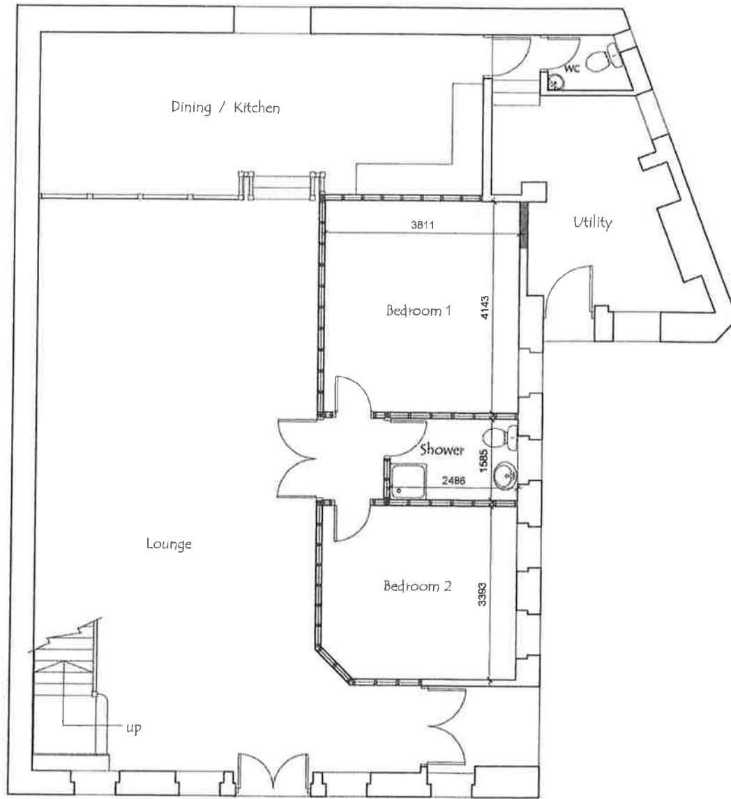
Proposed Ground Floor Layout Plan
