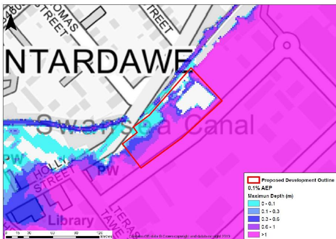
Figure 4-2 Post-developed 0.1% AEP maximum flood depths
