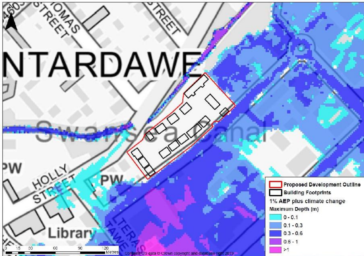
Figure 4-4 Post-developed 1% AEP plus climate change maximum flood depths
