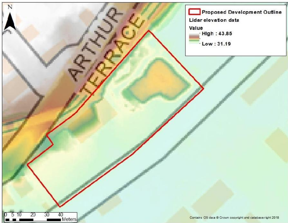
Figure 2-2 LiDAR elevation data
