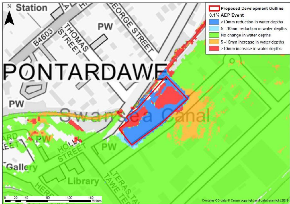
Figure 4-7 Pre-developed v post-developed 0.1% AEP
