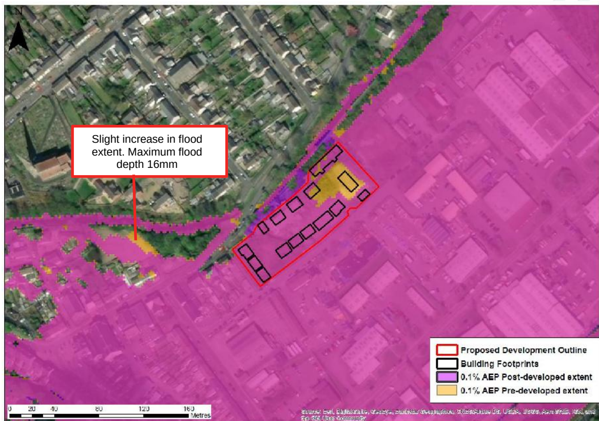
Figure 4-8 0.1% AEP pre-developed and post-developed flood extent
