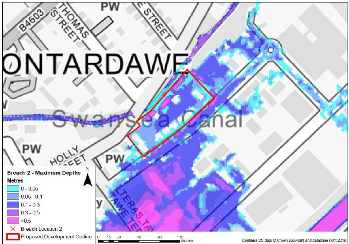
Figure 4-10: Breach 2: Maximum depth
