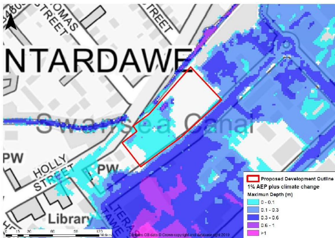
Figure 4-1 Pre-developed 1% AEP plus climate change maximum flood depths
