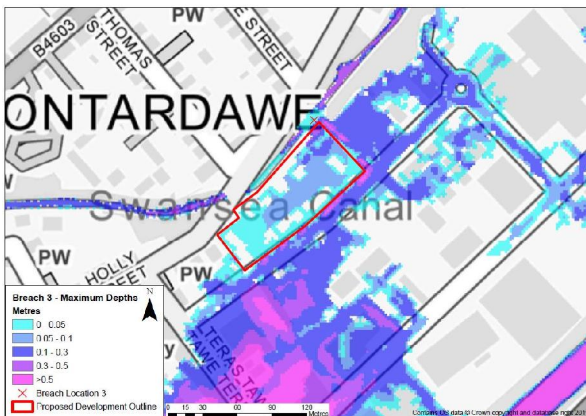
Figure 4-11: Breach 3: Maximum depth
