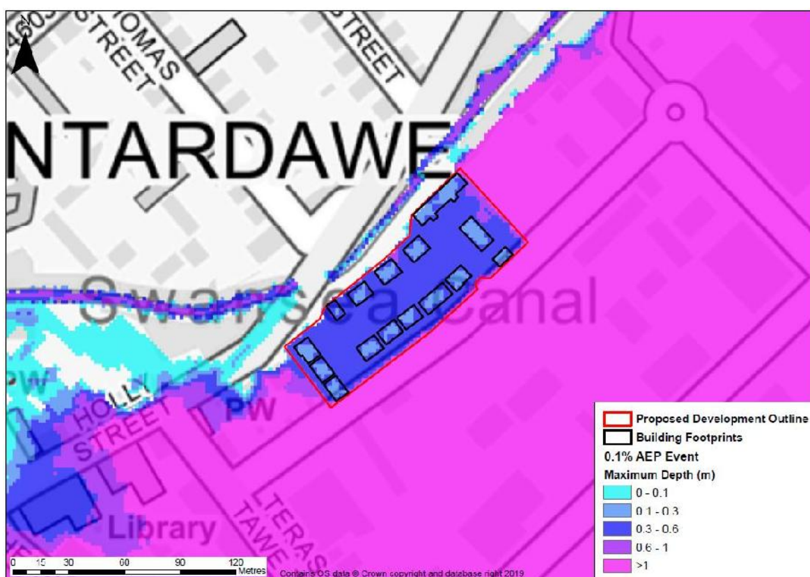
Figure 4-5 Post-developed 0.1% AEP maximum flood depths
