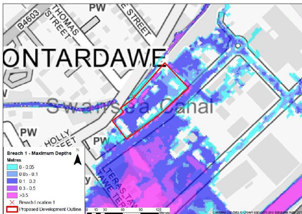
Figure 4-9: Breach 1: Maximum depth
