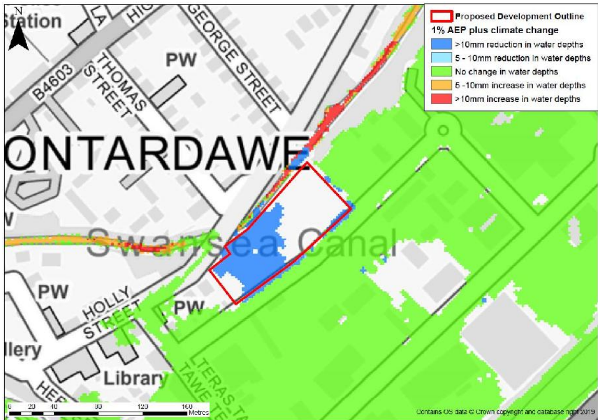
Figure 4-6 Pre-developed v post-developed 1% AEP plus climate change
