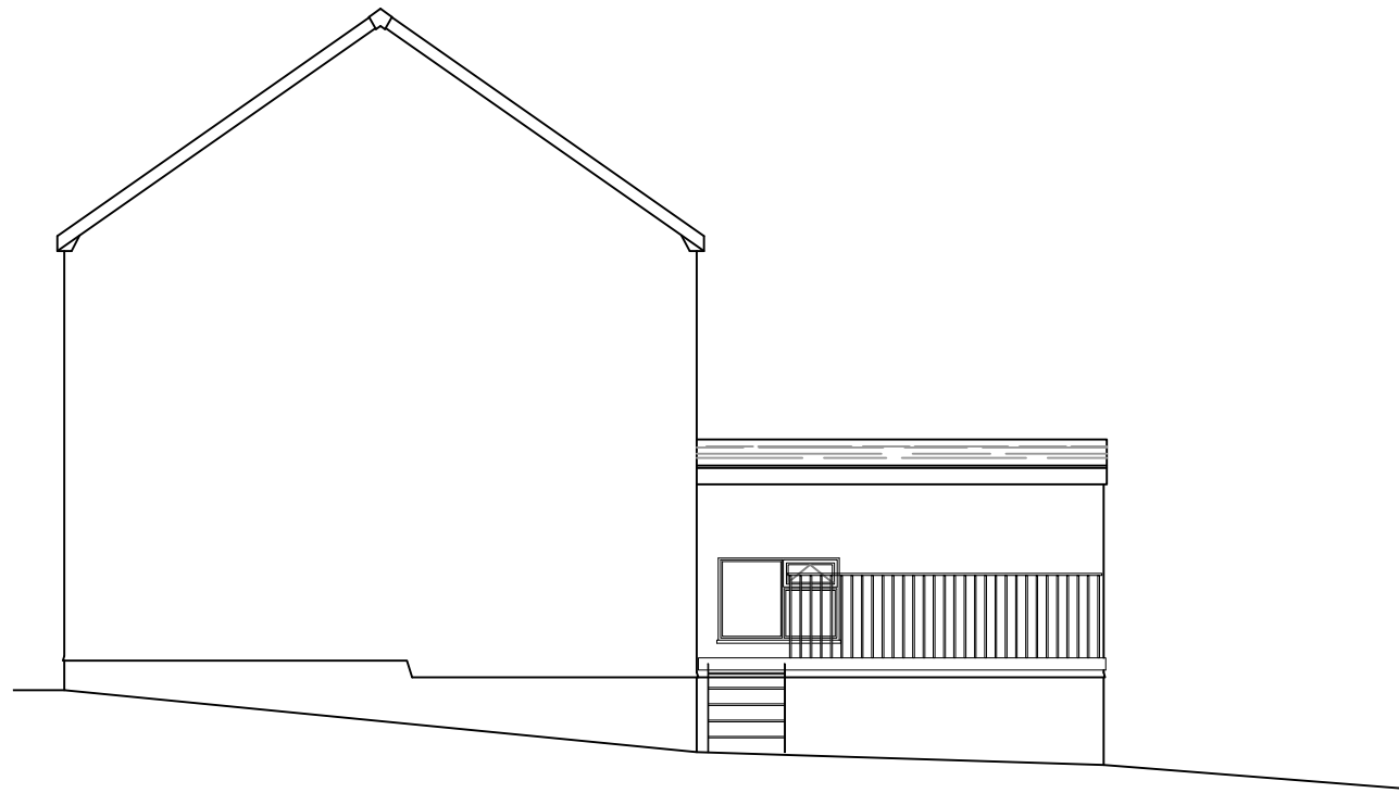
Existing elevation on 'A' Scale - 1:100
