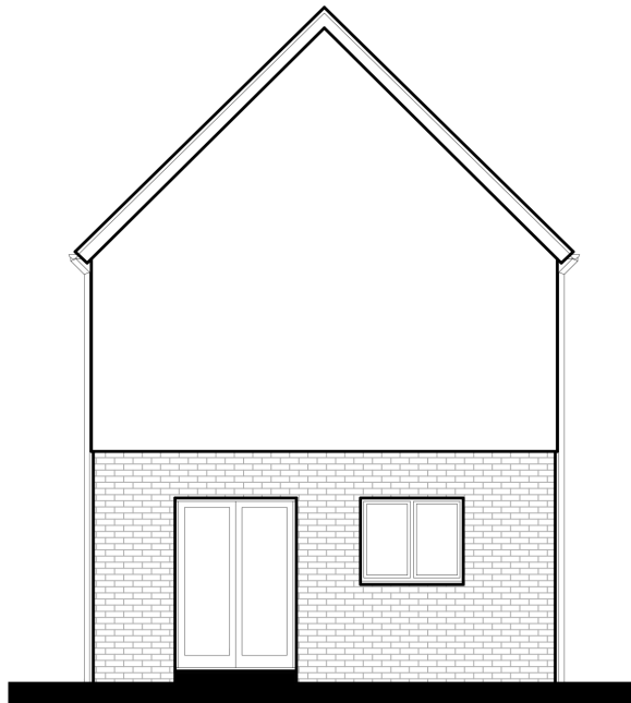
Side Elevation
