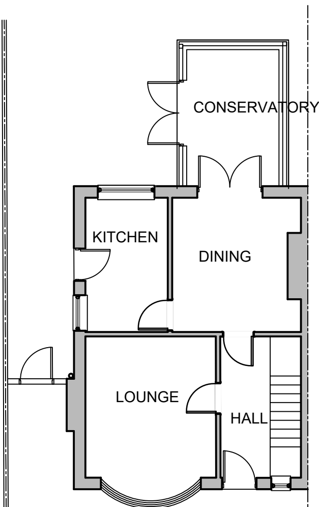
GROUND FLOOR PLAN AS EXISTING
