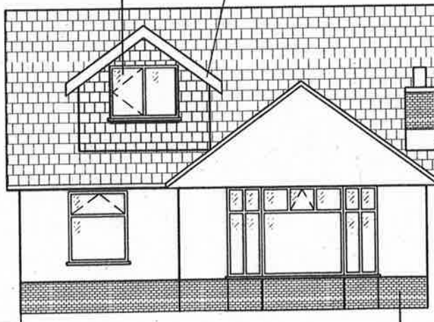
PROPOSED FRONT ELEVATION 1:50
