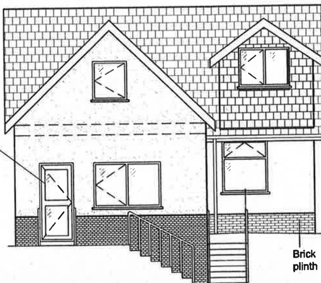
PROPOSED REAR ELEVATION 1:50
