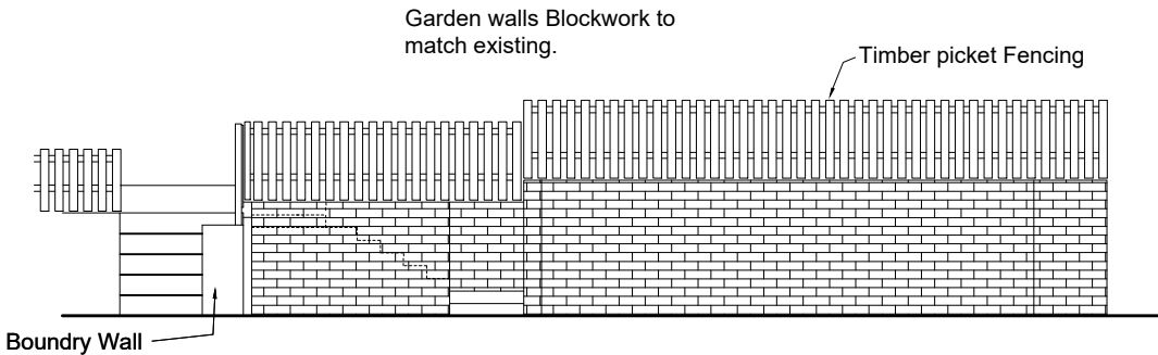
Proposed Elevation of Garden Steps and Wall
