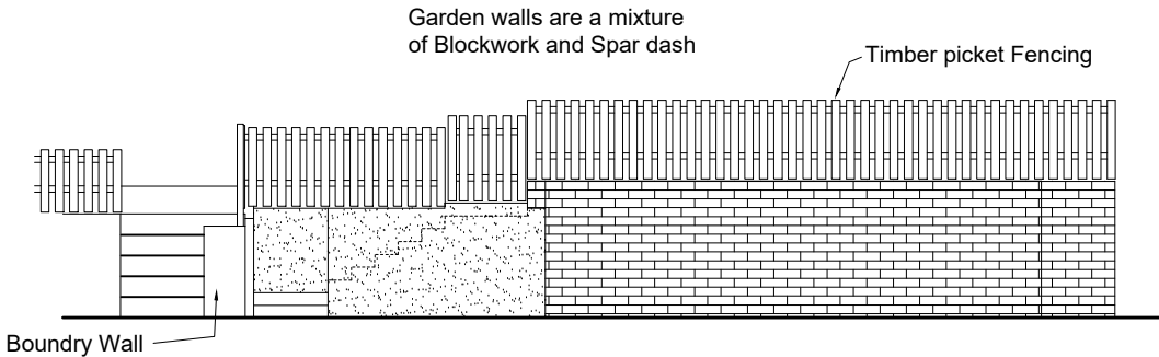
Existing Elevation of Garden Steps and Wall
