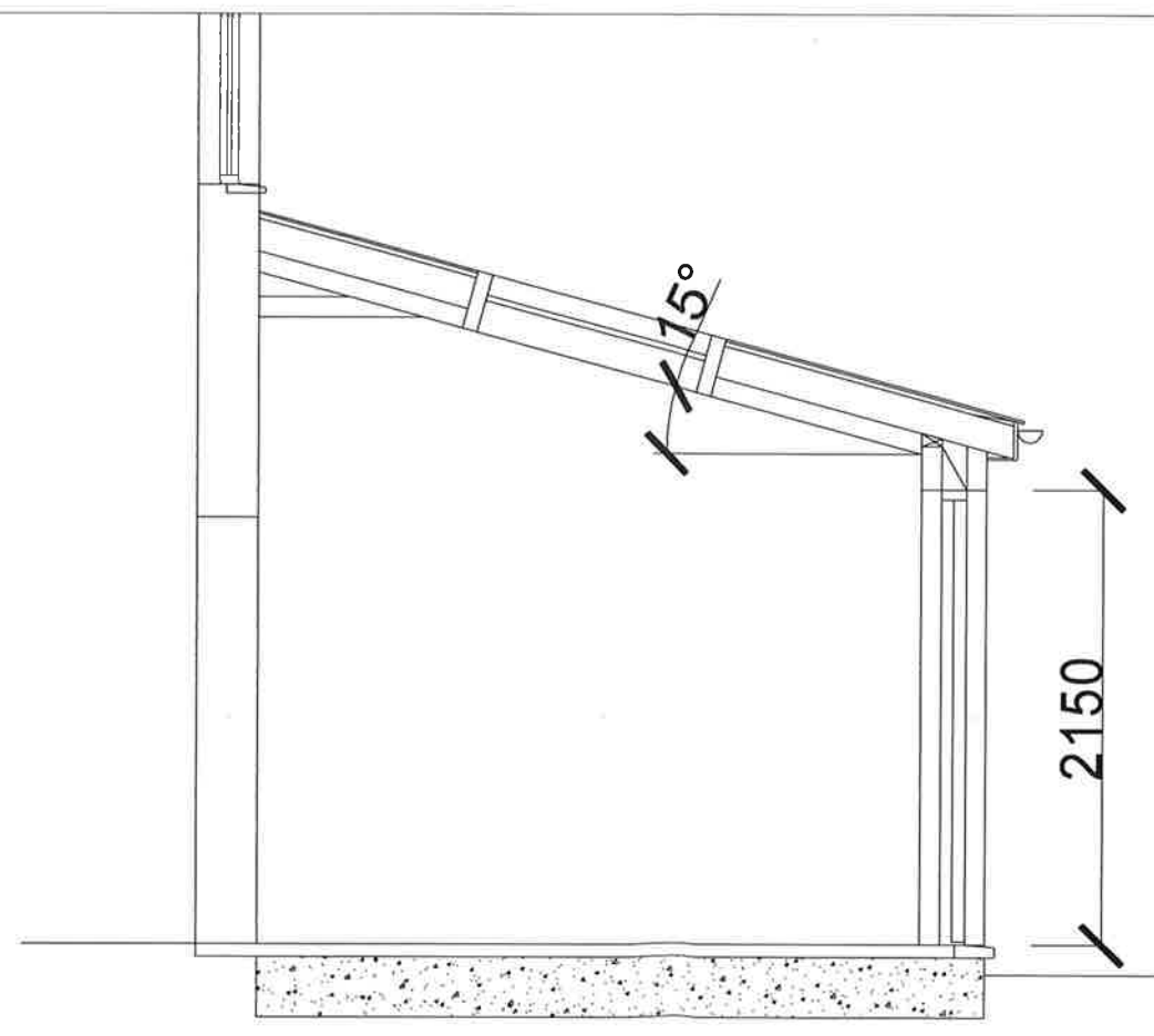
PROPOSED SECTION
