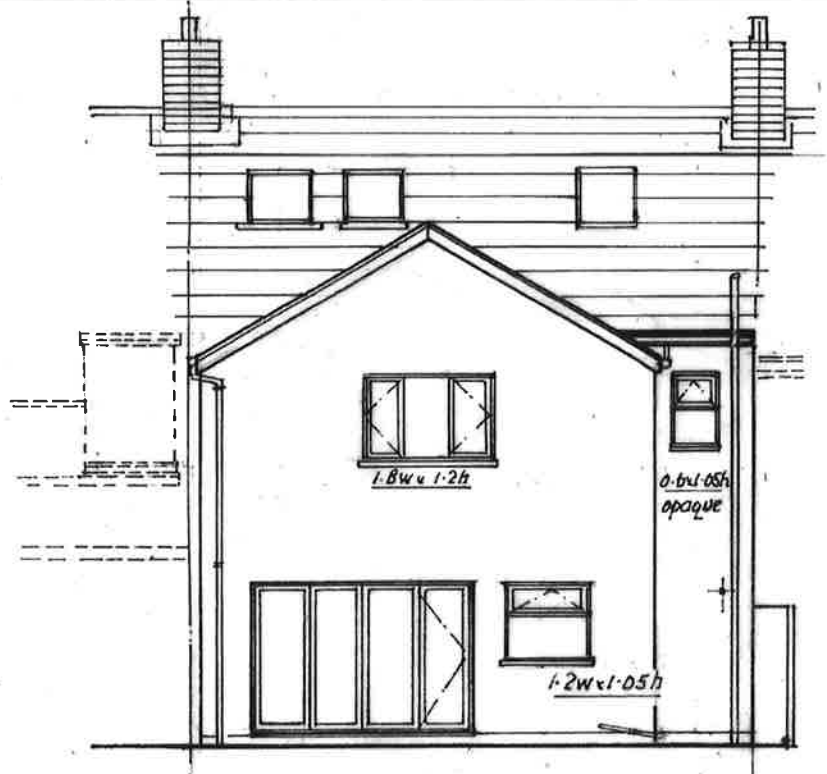
REAR ELEVATION
