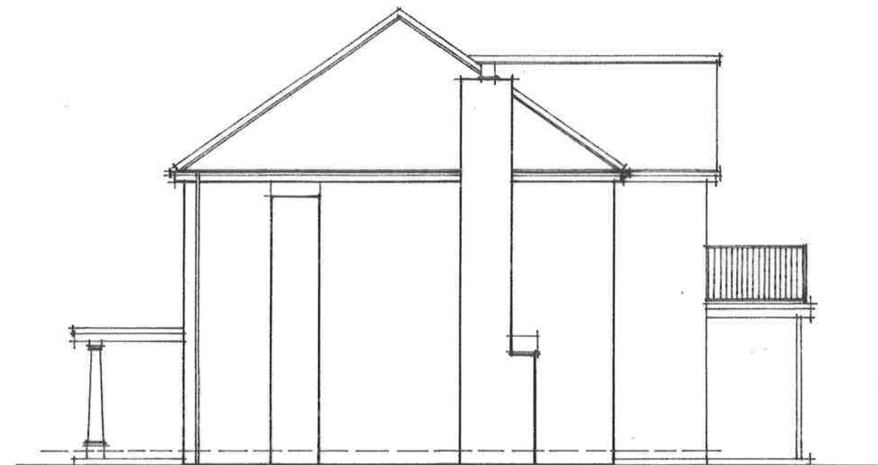
SIDE ELEVATION
