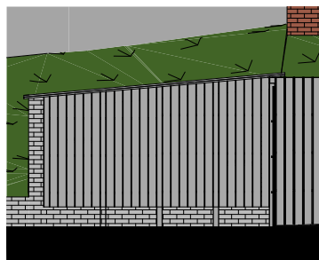
BS/2 - Left-Side Elevation 1:100
