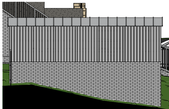
B/S1 - Rear Elevation 1:100
