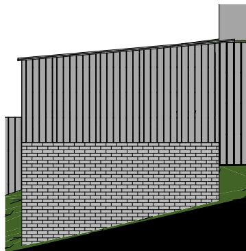
B/S1 - Left-Side Elevation 1:100
