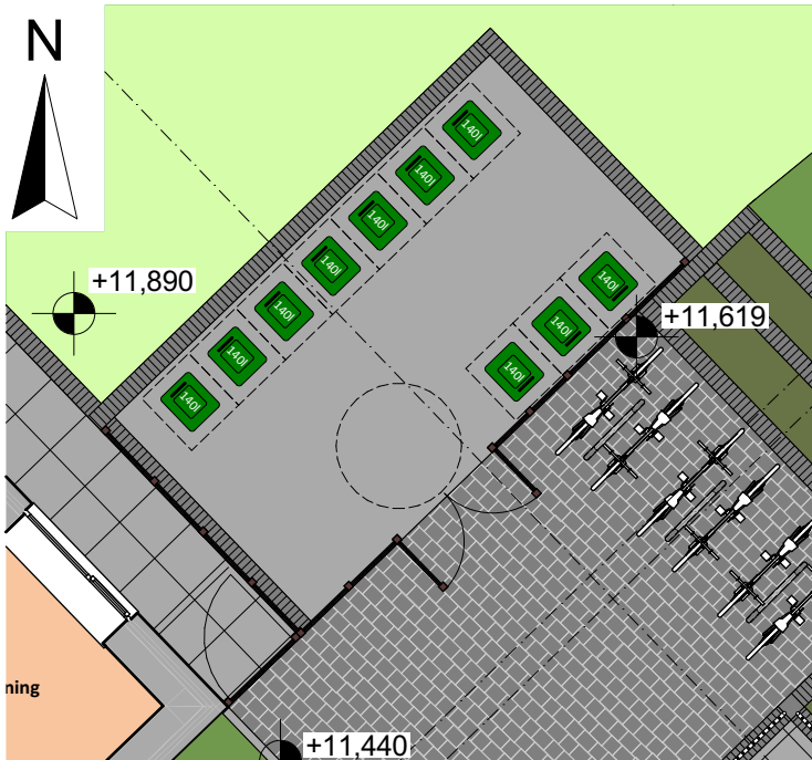
Bin Store 2 - Floor Plan 1:100
