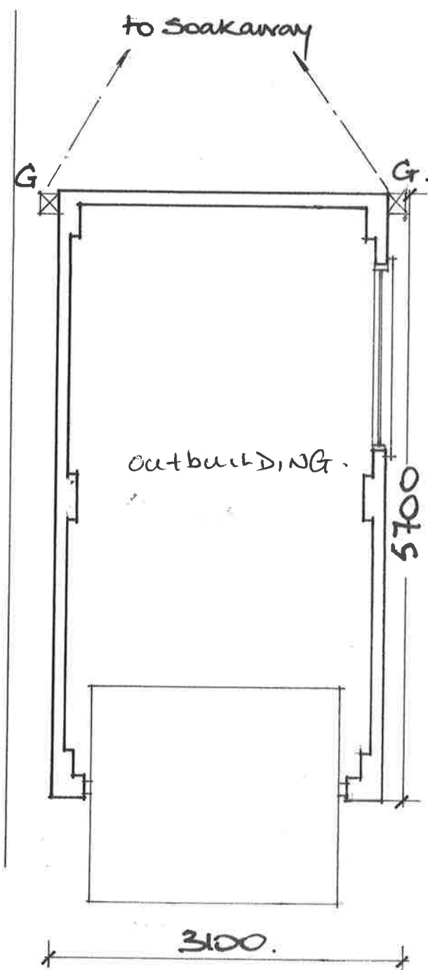
Plan View
