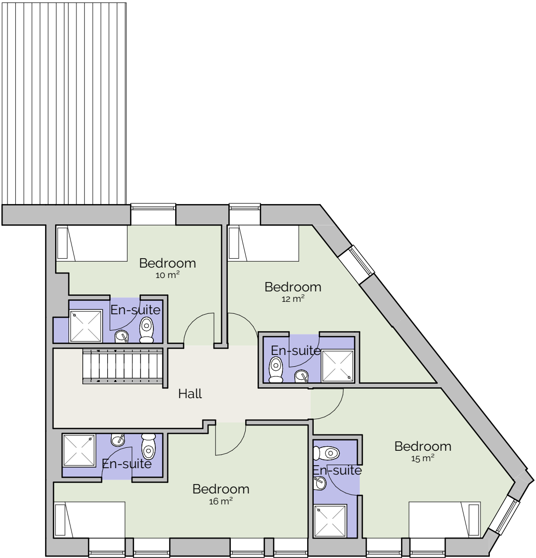
2 First Floor 1 : 100
