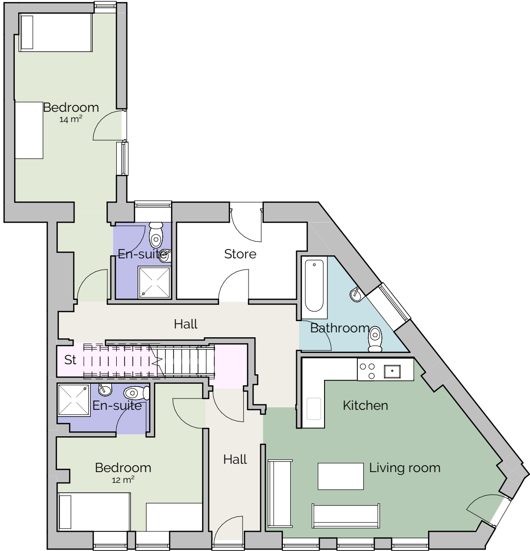
1 Ground Floor 1 : 100
