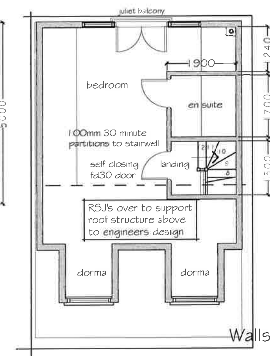
Proposed Loft Room Plan
