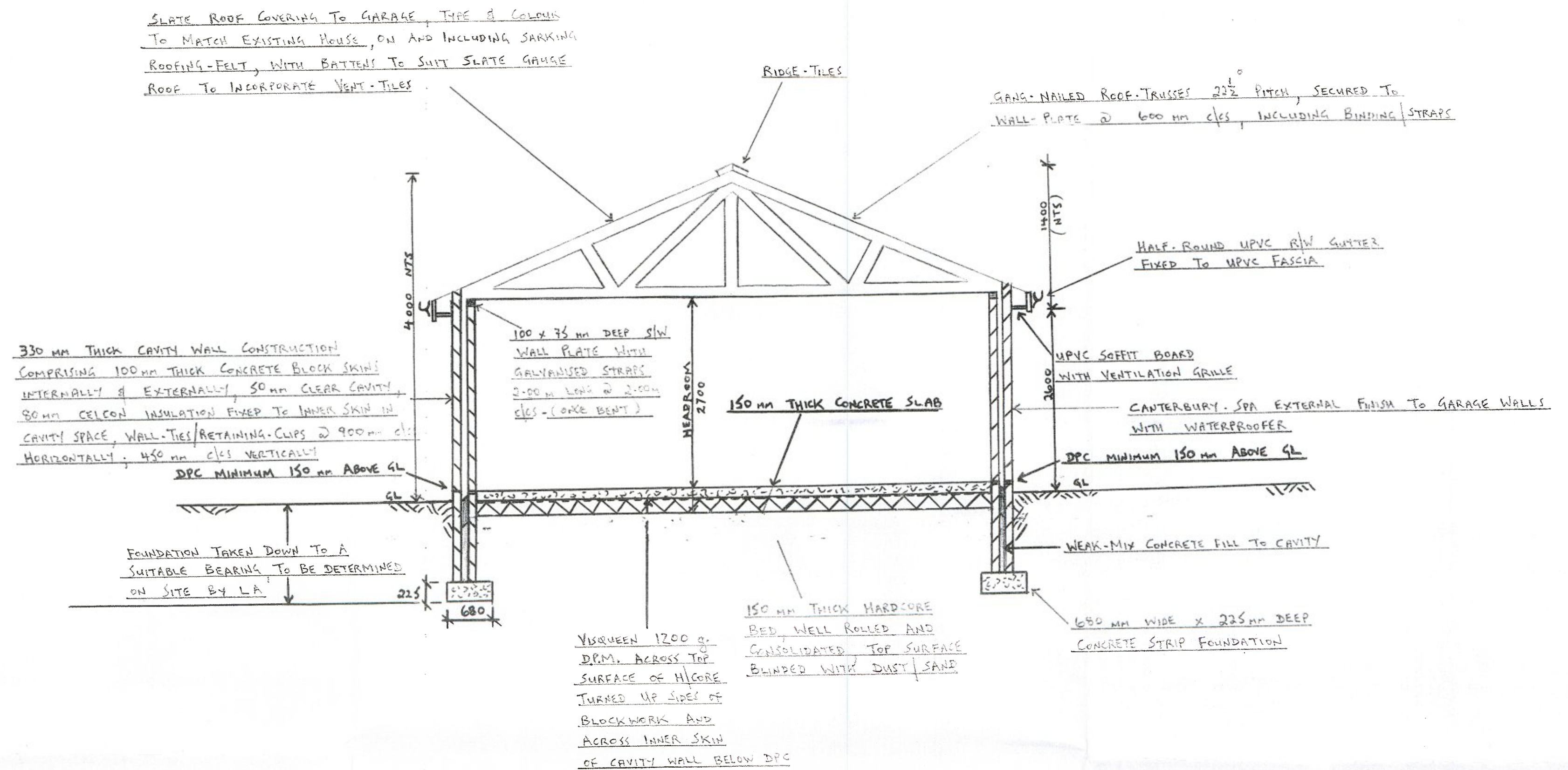
SECTION
