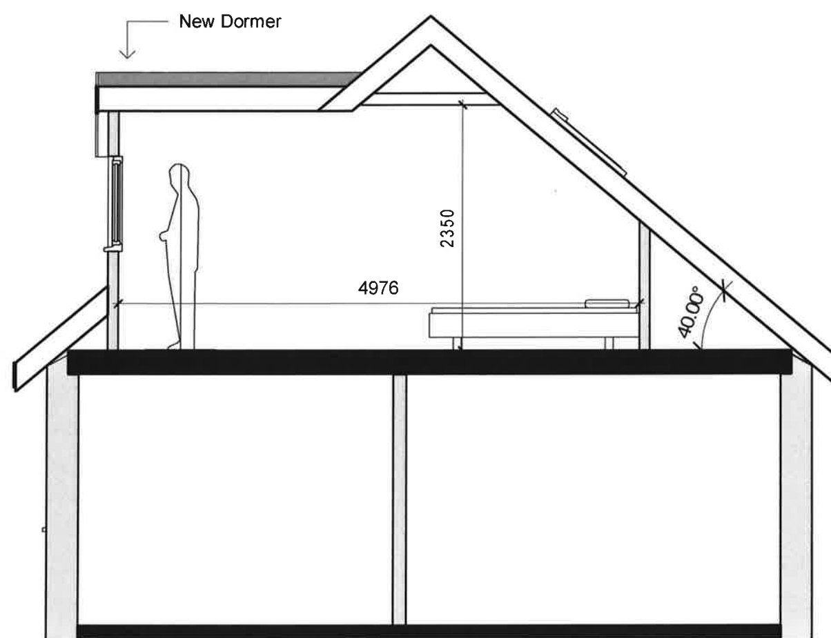
Proposed Section 2 1 : 50
