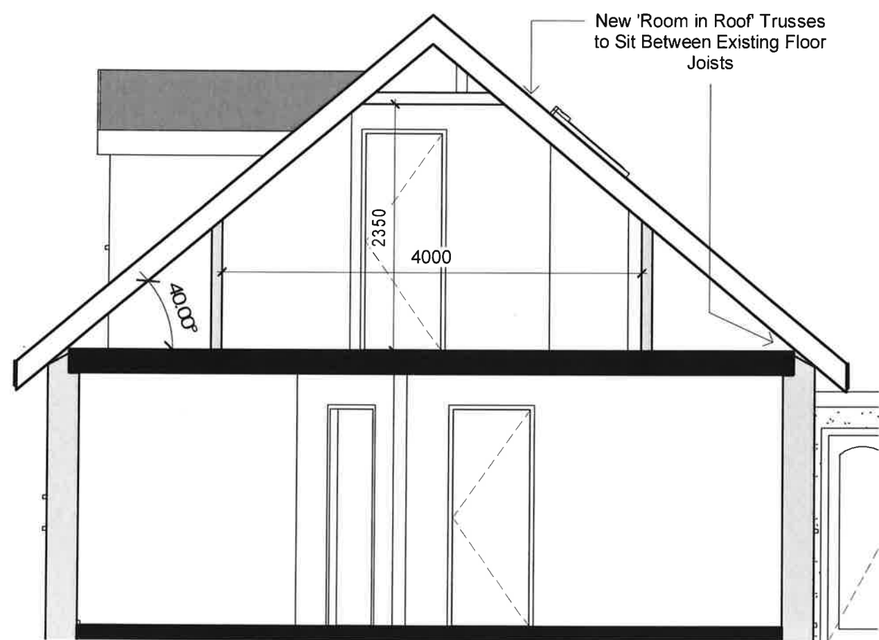
Proposed Section 1 1 : 50
