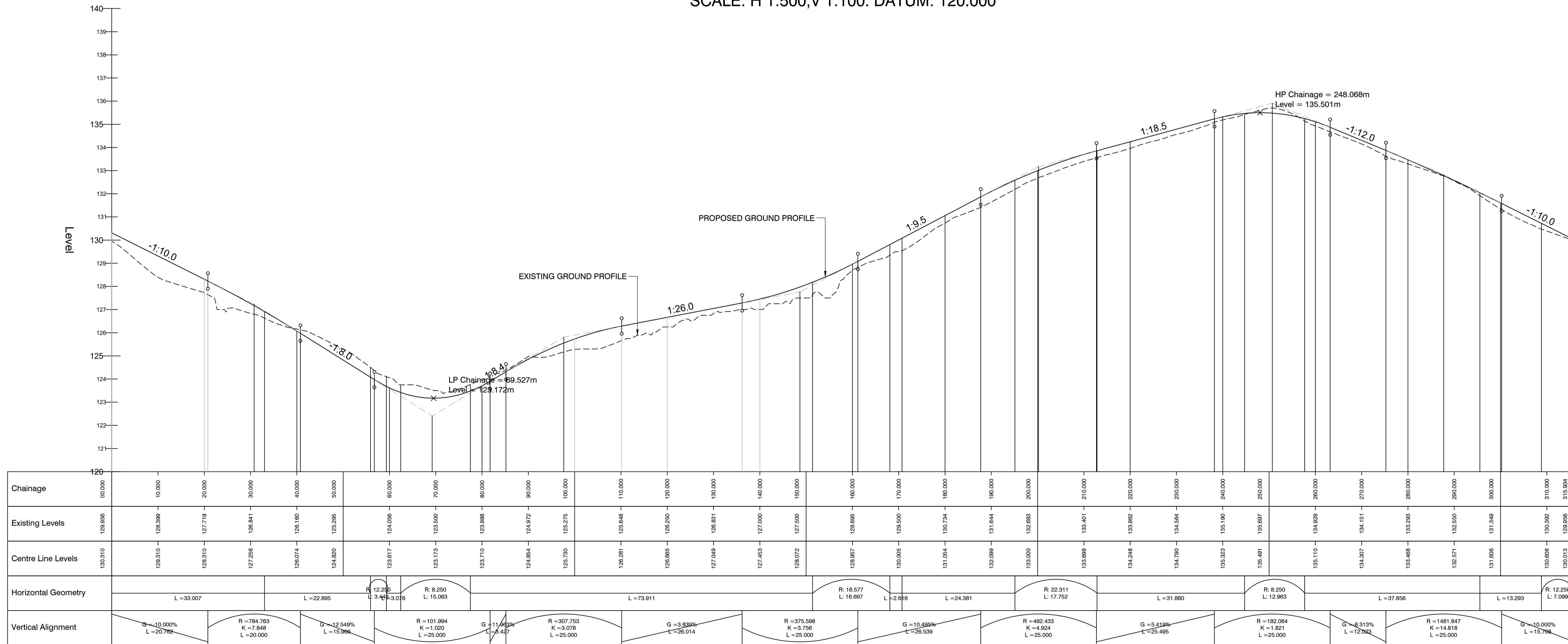
ROAD - 16-09-2019 - LONGSECTION SCALE: H 1:500,V 1:100. DATUM: 120.000
