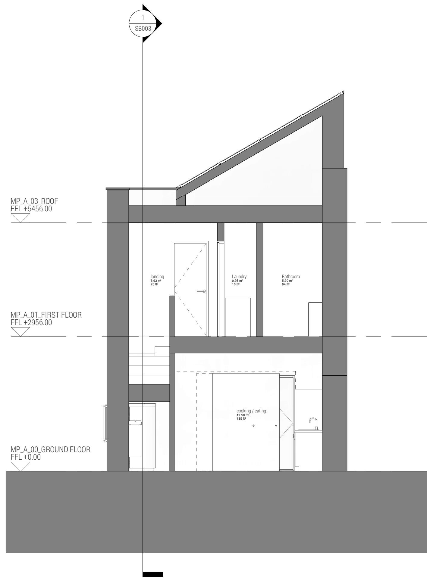
2 | Section 02
