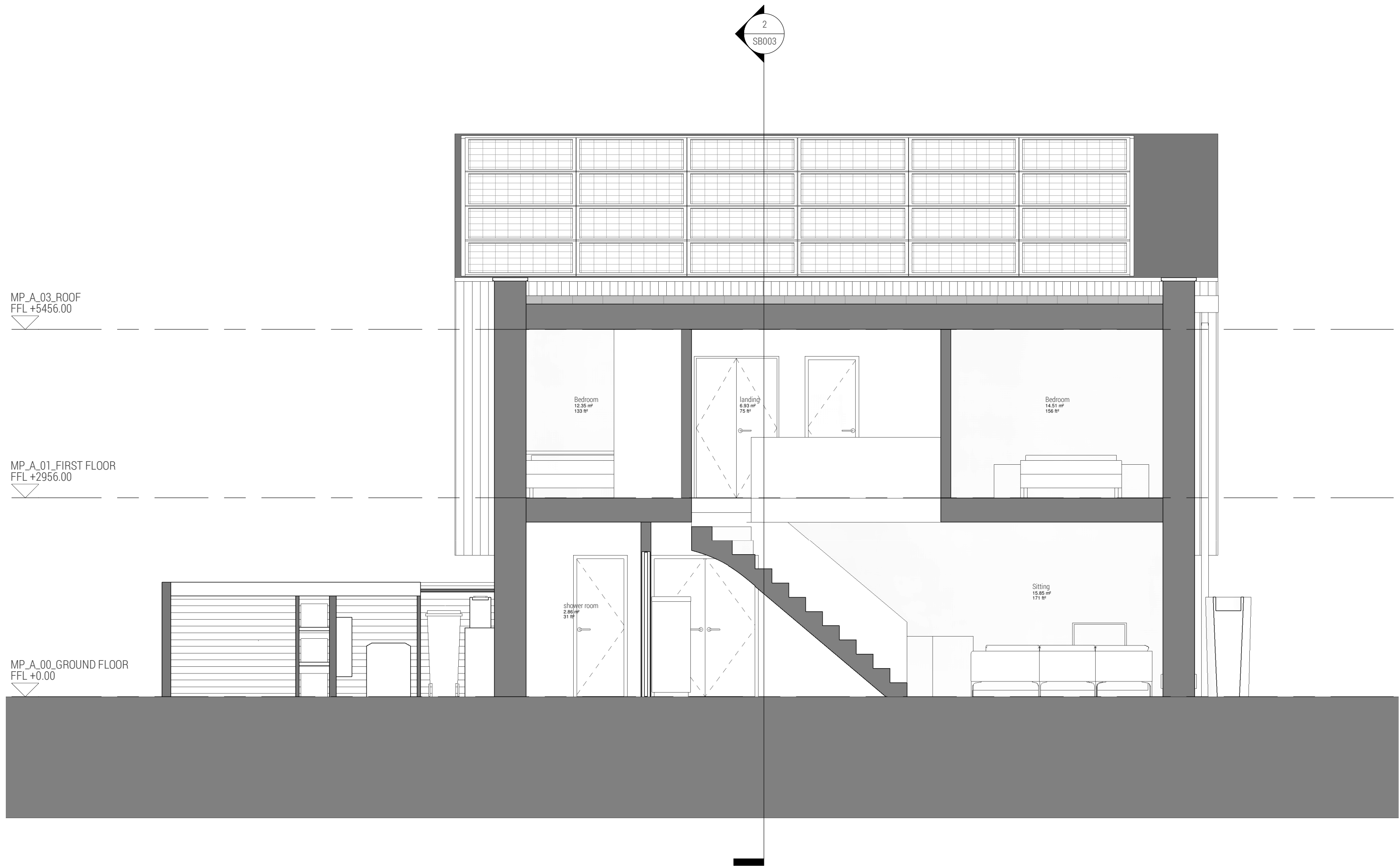
1 | Section 01
